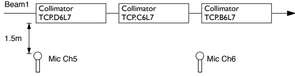
Figure 2: Positions of the microphones installed at the tunnel wall close to primary collimators in IR7 for beam 1.
