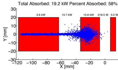
Figure 1: Power distribution on the face of the radiation absorber for the high luminosity layout.
