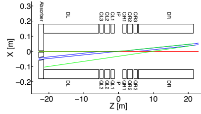
Figure 2: Radiation envelope for the high luminosity layout.
