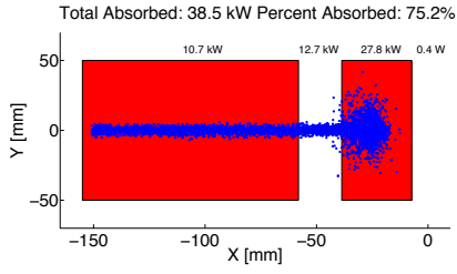
Figure 3: Power distribution on the face of the radiation absorber for the high acceptance layout.
