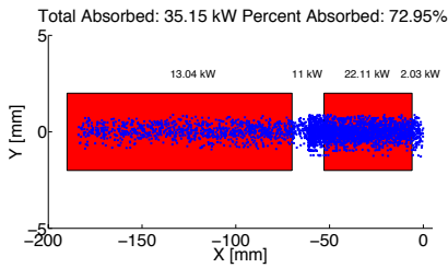
Figure 5: Power distribution on the face of the radiation absorber for the linac-ring design.
