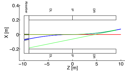
Figure 6: Radiation envelope for the linac-ring design.
