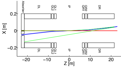
Figure 4: Radiation envelope for the high acceptance layout.
