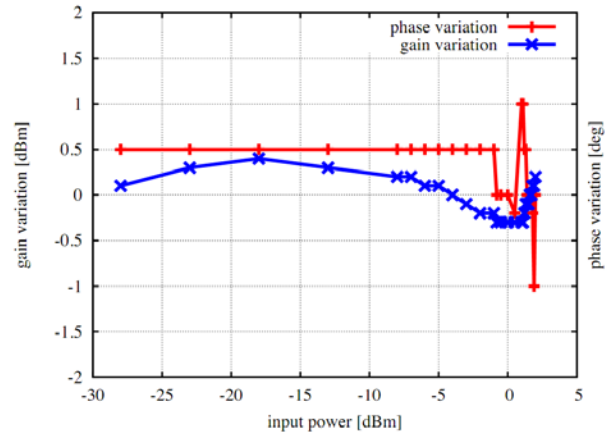
Figure 5: Phase and amplitude gain variation
