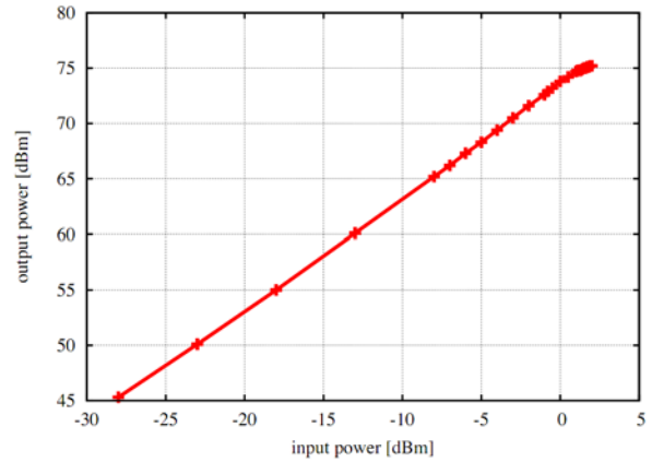
Figure 4: Output versus input power
