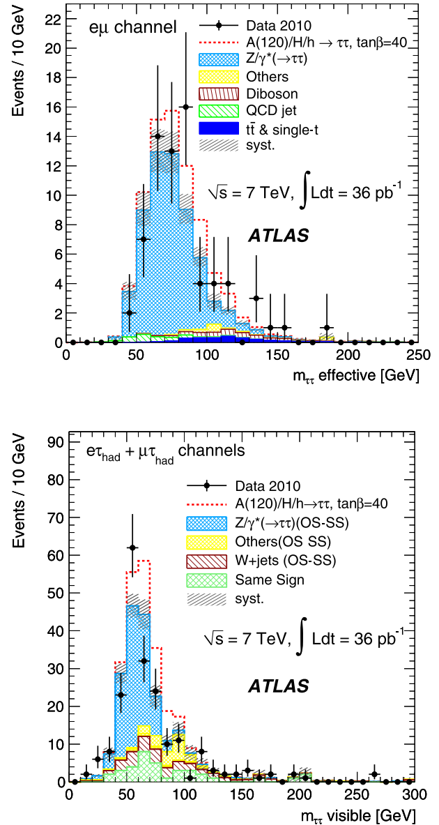
Fig. 1. Effective mass distribution for the e\mu final state (top) and visible mass distribution for \ell\tau_{had} final states (bottom). The data are compared with the background expectation and an added hypothetical signal. “OS-SS” denotes the difference between the opposite-sign and same-sign event yields. Further explanations are given in the text.
