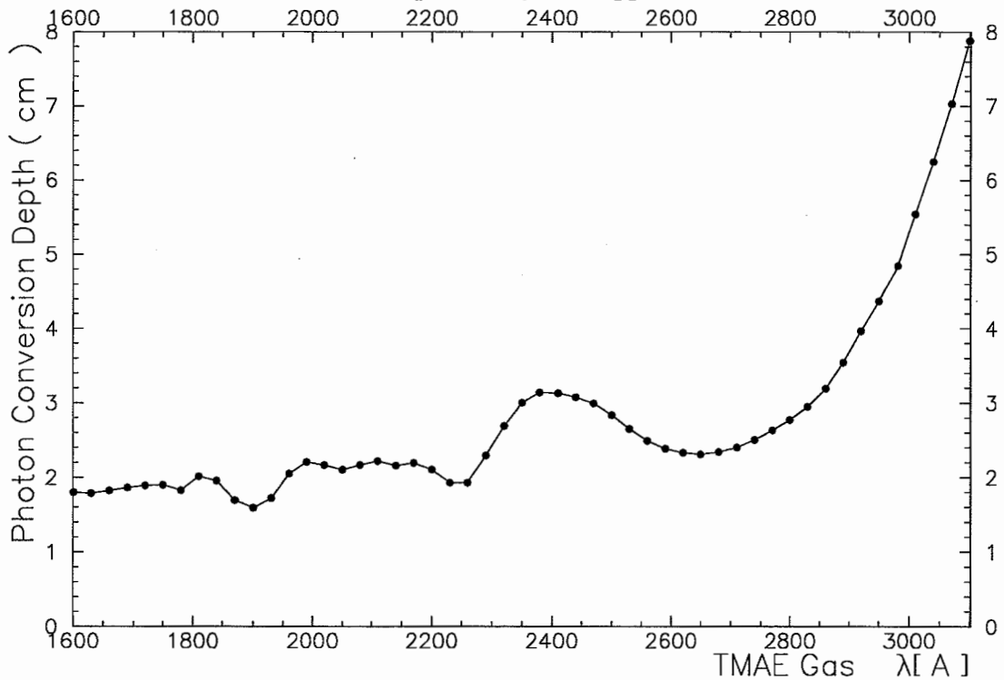
Figure 3: Photon conversion depth vs wavelength of the Barrel RICH photon detector. The TMAE saturated vapour temperature is 28^\circ\text{C} in 75/25% CH_4/C_2H_6 drift gas mixture.
