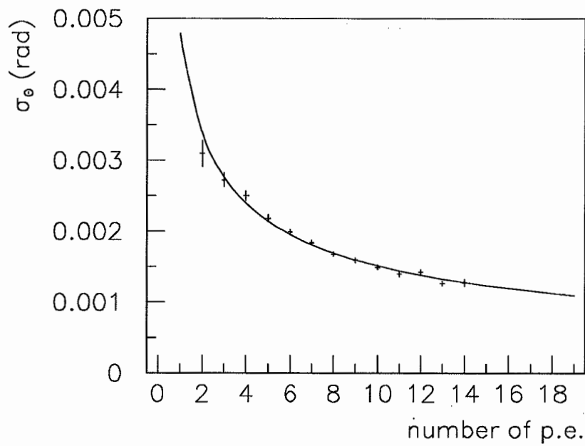
Figure 4: The mean Cherenkov angle resolution for the Barrel RICH gas radiator vs the number of detected photo-electrons per ring from 1993 Z^0 \rightarrow \mu^+\mu^- selected events.
