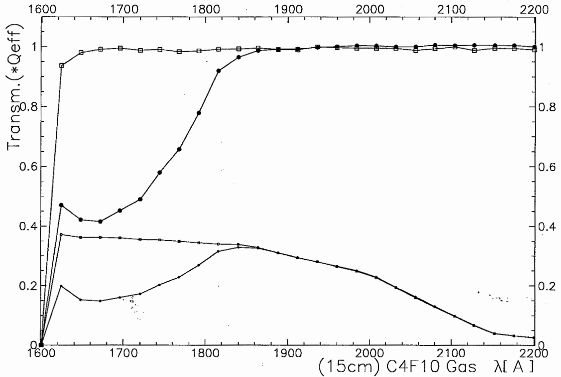
Figure 2: UV transmission vs wavelength (in Å) of the Forward RICH C_4F_{10} gas radiator.
