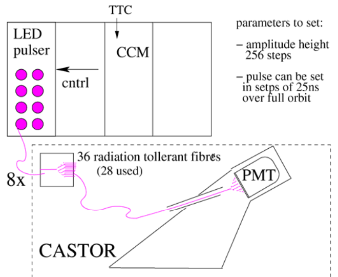
Figure 3 The LED monitoring system
