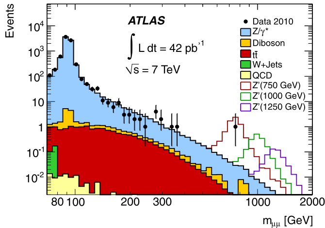
Fig. 2. Dimuon invariant mass ( m_{\mu^+\mu^-} ) distribution after final selection, compared to the stacked sum of all expected backgrounds, with three example Z'_{SSM} signals overlaid. The bin width is constant in \log m_{\mu^+\mu^-} and the ratio of the upper to lower bounds of each bin is 1.07.
