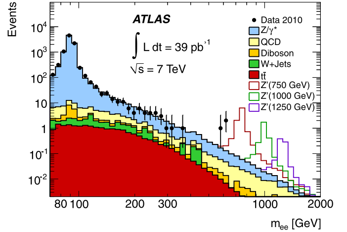
Fig. 1. Dielectron invariant mass ( m_{e^+e^-} ) distribution after final selection, compared to the stacked sum of all expected backgrounds, with three example Z'_{\text{SSM}} signals overlaid. The bin width is constant in \log m_{e^+e^-} and the ratio of the upper to lower bounds of each bin is 1.07.
