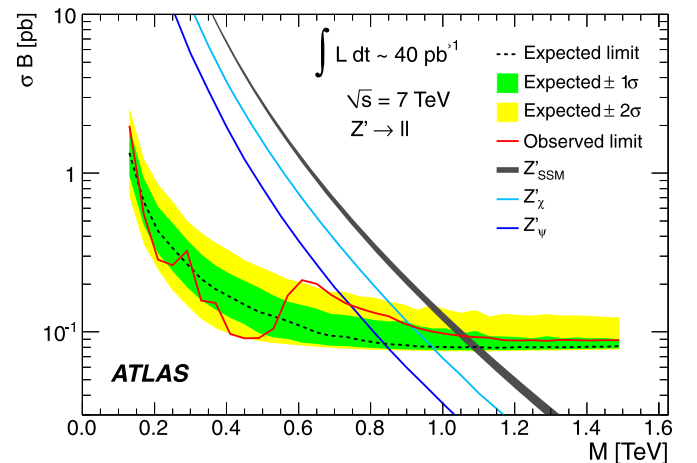
Fig. 5. Expected and observed 95% C.L. limits on \sigma B and expected \sigma B for Z'_{SSM} production and the two E_6 -motivated Z' models with lowest and highest \sigma B for the combination of the electron and muon channels. The thickness of the Z'_{SSM} theory curve represents the theoretical uncertainty and holds for the other theory curves.
