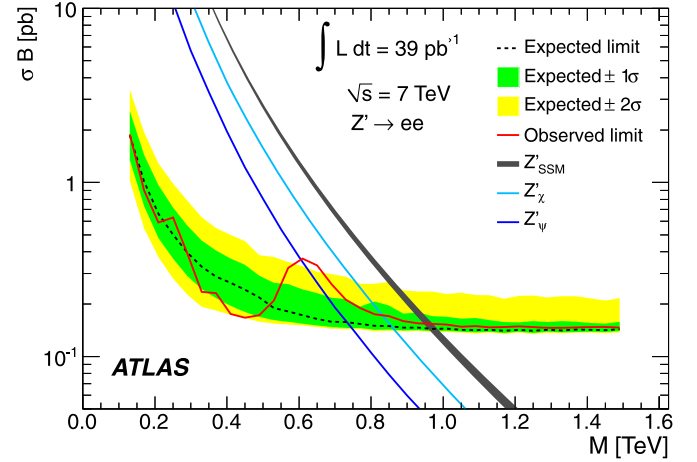
Fig. 3. Expected and observed 95% C.L. limits on \sigma B and expected \sigma B for Z'_{SSM} production and the two E_6 -motivated Z' models with lowest and highest \sigma B for the dielectron channel. The thickness of the SSM theory curve represents the theoretical uncertainty and holds for the other theory curves.
