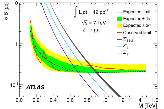
Fig. 4. Expected and observed 95% C.L. limits on \sigma B and expected \sigma B for Z'_{SSM} production and the two E_6 -motivated Z' models with lowest and highest \sigma B for the dimuon channel. The thickness of the SSM theory curve represents the theoretical uncertainty and holds for the other theory curves.
