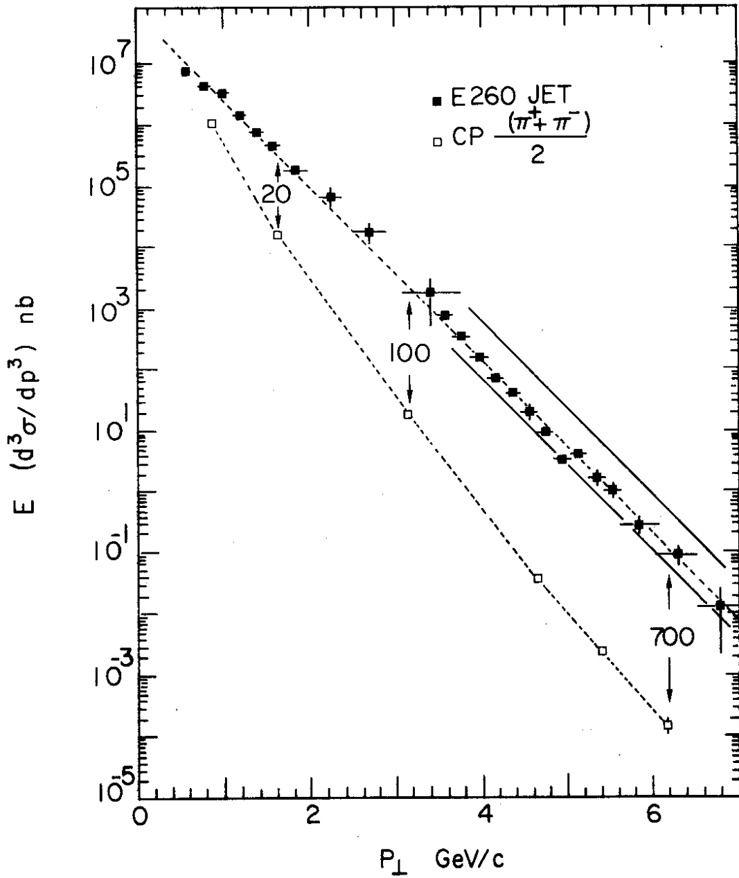
Figure 6 : Inclusive distribution for jets and for single particles. The jet data are from the Caltech-UCLA-Fermilab-Illinois Collaboration. The QCD calculation for jet production at fixed jet energy and fixed jet momentum brackets the data : G. Fox, private communication.
