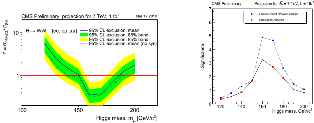
Figure 2: Expected significance for the H \rightarrow WW \rightarrow 2\ell 2\nu channel as a function of m_H , for \sqrt{s} = 7 TeV and L = 1 fb ^{-1} .
