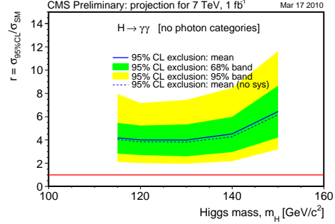
Figure 4: Exclusion plot for the H \rightarrow \gamma\gamma channel, for \sqrt{s} = 7 TeV and L = 1 fb ^{-1} .
