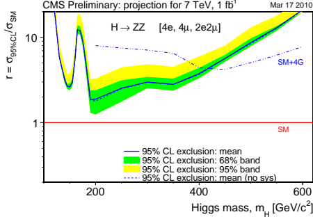
Figure 3: Exclusion plot for the H \rightarrow ZZ \rightarrow 4\ell channel, for \sqrt{s} = 7 TeV and L = 1 fb ^{-1} .
