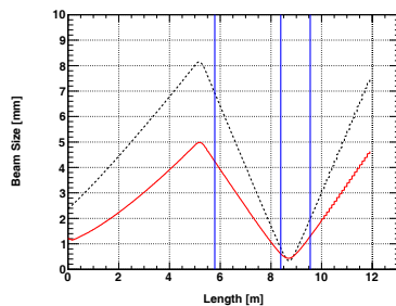
Figure 2: Variation of beam sizes along the Linac4 dump line (horizontal/vertical measurement: dotted/solid line). The three screen positions are marked with vertical lines.
