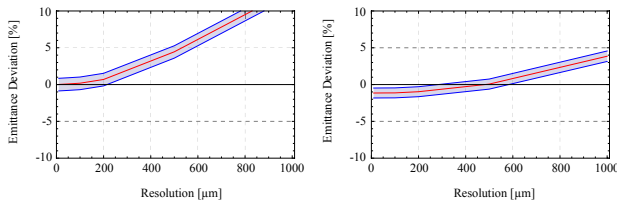
Figure 3: Deviation of the reconstructed emittance referred to its reference value at monitor 1 versus different (common) resolutions of the beam size measurement (left: horizontal plane, right: vertical plane). The central line indicates the nominal reconstructed value determined from the fitted beam sizes, while the error band shows the maximum deviations from the nominal value if the fitted beam sizes are systematically varied by their fit parameter error.
