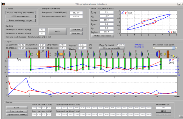
Figure 1: Graphical user interface showing the beam transmission and trajectory as well as the beta functions of the matched beam.
