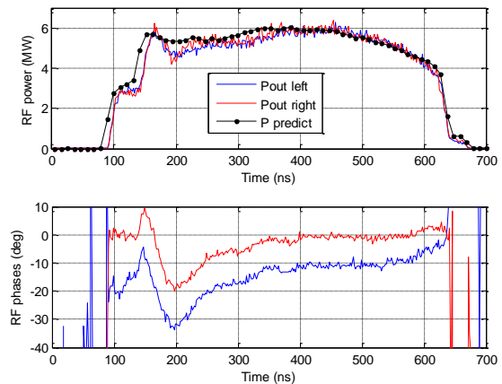
Figure 2: PETS output power measurement and prediction from the BPM signal (upper) and the corresponding phase of the rf signal (lower).
