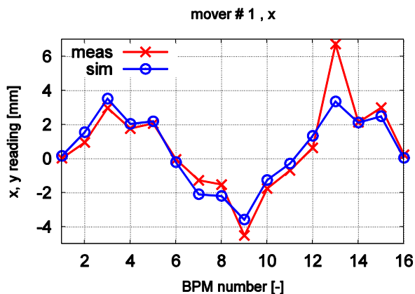
Figure 3: Kick measurement using the mover of the first quadrupole in the horizontal plane. The measured beam trajectory is compared to the optics simulations.
