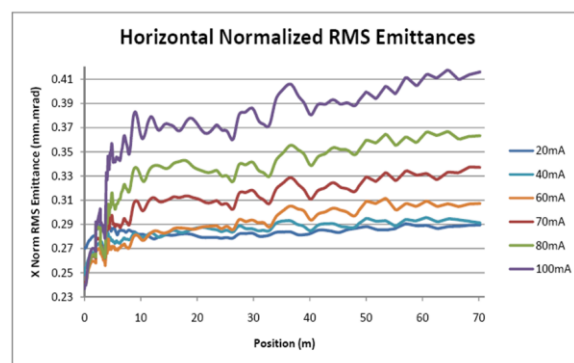
Figure 2: Horizontal RMS emittance evolution from MEBT to PIMS for different beam currents.
