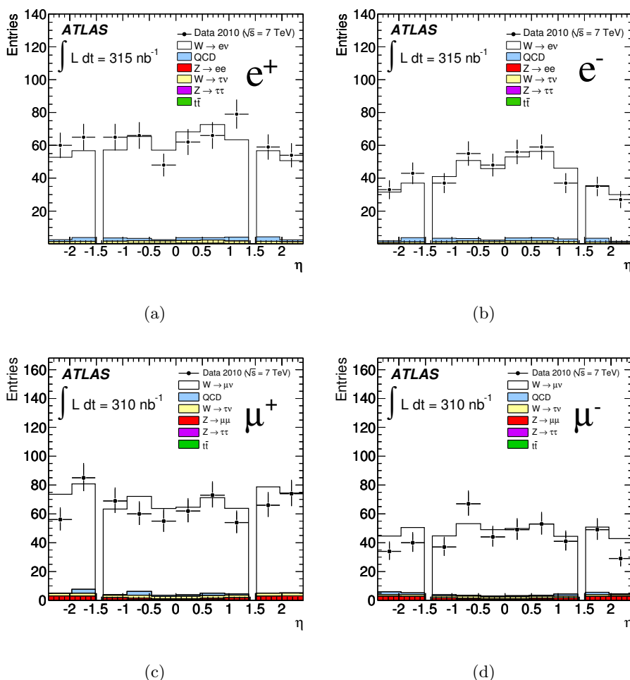
Figure 15. Pseudorapidity distributions of e^+ (a), e^- (b), \mu^+ (c) and \mu^- (d) candidates satisfying all W requirements (see section 5.4). The data are compared to the Monte Carlo simulation, broken down into the signal and various background components. The Monte-Carlo distributions are normalised to the integrated luminosity of the data, as described in section 5.2. The values of the integrated luminosities for the two channels have uncertainties of \pm 11\% , see section 3.
