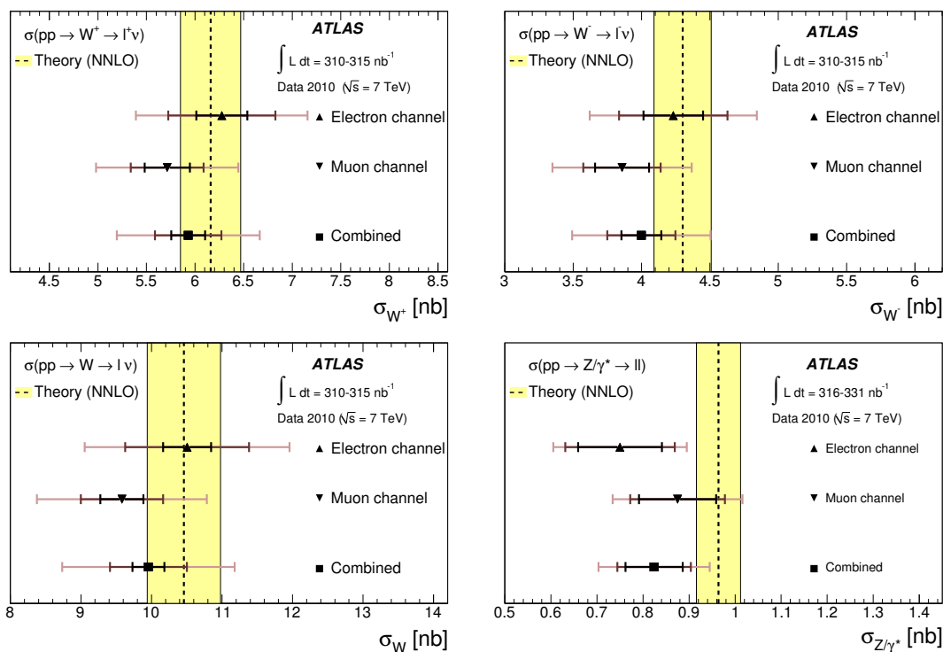
Figure 11. The measured values of \sigma_W \cdot \text{BR}(W \rightarrow l\nu) for W^+ , W^- and for their sum and of \sigma_{Z/\gamma^*} \cdot \text{BR}(Z/\gamma^* \rightarrow ll) compared to the theoretical predictions based on NNLO QCD calculations (see text). Results are shown for the electron and muon final states as well as for their combination. The error bars represent successively the statistical, the statistical plus systematic and the total uncertainties (statistical, systematic and luminosity). All uncertainties are added in quadrature. The quoted luminosity range spans the values used for the electron and muon channels. The systematic uncertainty on these numbers is \pm 11\% , see section 3.
