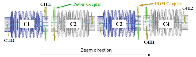
Figure 2: Schematic representation of 4 cavities within ACC39. The power couplers are indicated in green, and the HOM couplers are indicated in brown.
