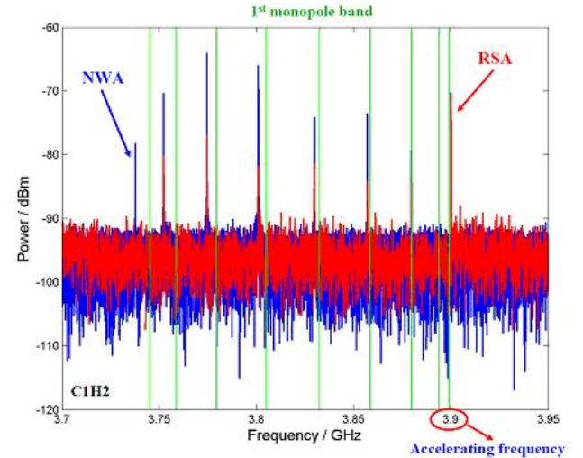
Figure 4: Comparison of spectrum taken by RSA (concatenation of two spectra) and NWA (transmission measurement without beam-excitation) of C1H2. The vertical lines indicate the simulation results.
