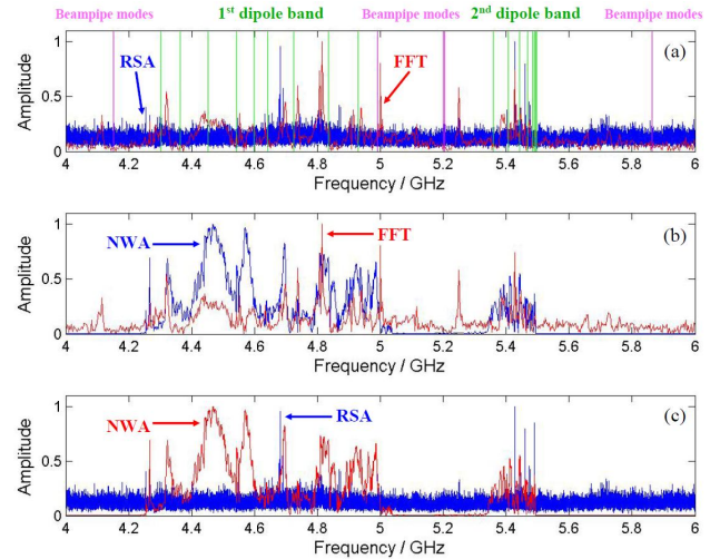
Figure 5: Comparison of spectra taken by Scope (after FFT), RSA (after concatenation) of C1H1 and NWA (transmission measurement without beam-excitation). The vertical lines indicate the simulation results. All spectra are normalized to the highest amplitude in frequency span of 4 GHz to 6 GHz.
