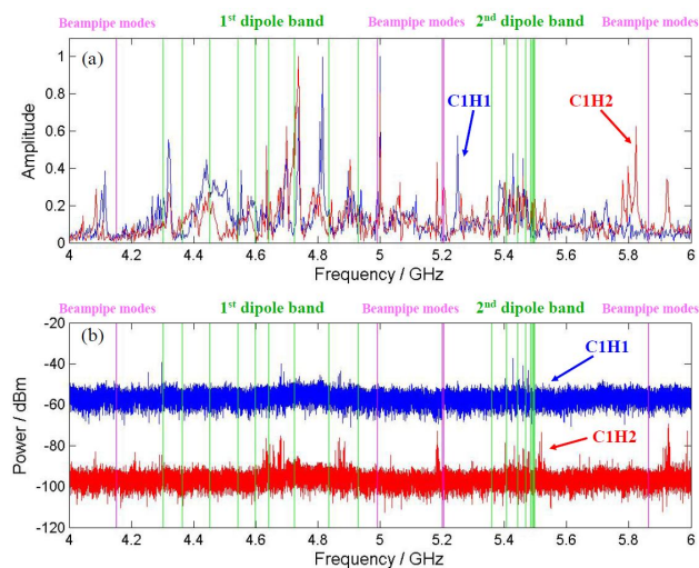
Figure 6: Comparison of spectra taken from C1H1 and C1H2 by using Scope (a) (after FFT) and RSA (b) (after concatenation). The vertical lines indicate the simulation results. (a) is normalized to the highest amplitude in frequency span of 4 GHz to 6 GHz; (b) 40 dBm are added arbitrarily to C1H1 spectrum only for better comparisons.
