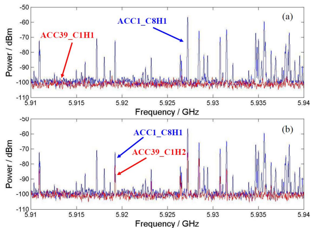
Figure 7: Transmissions from ACC1 to ACC39. Both C1H1 (a) and C1H2 (b) are compared to the last HOM coupler of last cavity (C8H1) of ACC1.
