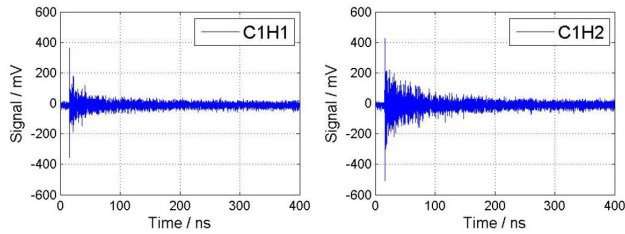
Figure 3: HOM signal from two HOM couplers of C1.
