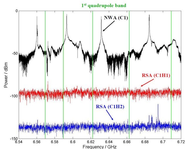
Figure 8: Comparison of spectrum taken by RSA (concatenation of two bunches) and NWA (transmission measurement) of C1H1 and C1H2. The vertical lines indicate the simulation results. 45 dB is added arbitrarily to NWA spectrum while 40 dBm is subtracted from C1H2 spectrum only for better comparisons.
