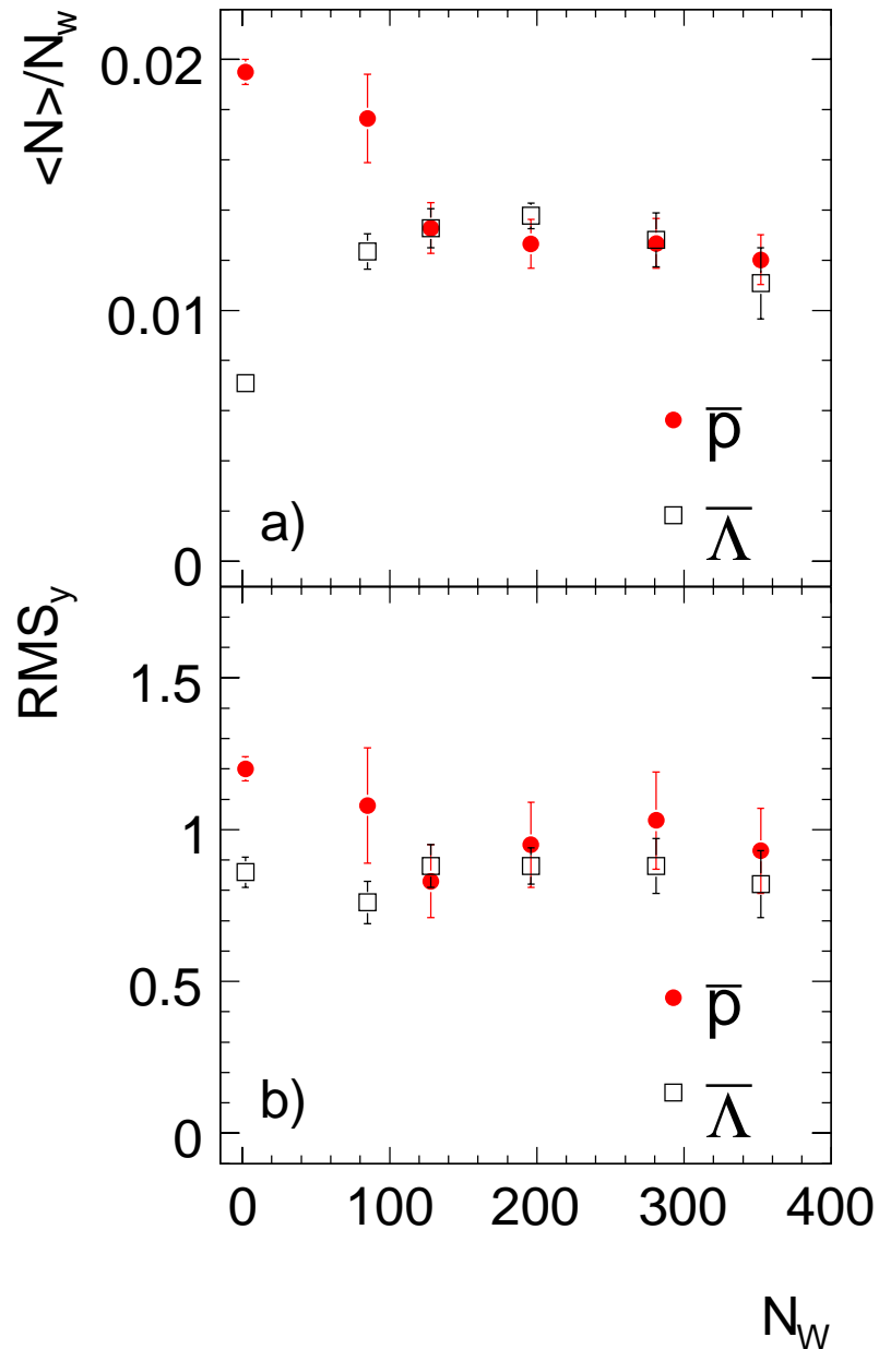
FIG. 8: The total multiplicities (per wounded nucleon) of \bar{p} and \bar{\Lambda} (upper panel) and the \text{RMS}_y widths of the dn/dy distributions of \bar{p} and \bar{\Lambda} (lower panel) for five centralities as function of the number of wounded nucleons \langle N_w \rangle in Pb+Pb collisions at 158A GeV. The \bar{\Lambda} data are from [21]. Also shown are results on antiprotons obtained from p+p interactions [22]. Only statistical errors are shown (if larger than the symbol size). For the systematic errors see section IIIC.
