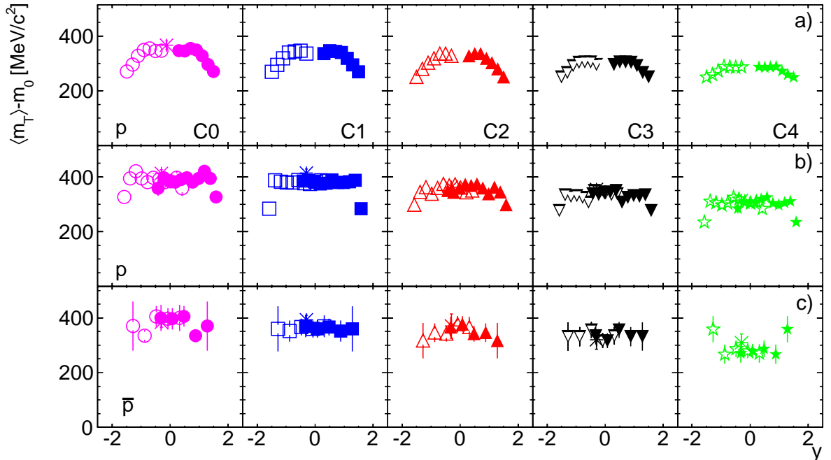
FIG. 4: \langle m_T \rangle - m_0 for (anti-)protons as function of rapidity for five centrality intervals in Pb+Pb collisions. We show in the upper row (a) protons at 40A GeV, in the middle row (b) protons at 158A GeV, and in the lower row (c) antiprotons at 158A GeV. The open symbols are obtained by reflection at mid-rapidity. Asterisks refer to results of an earlier analysis using TOF information for particle identification [5]. Only statistical errors are shown (if larger than the symbol size). For the systematic errors see section IIIC.
