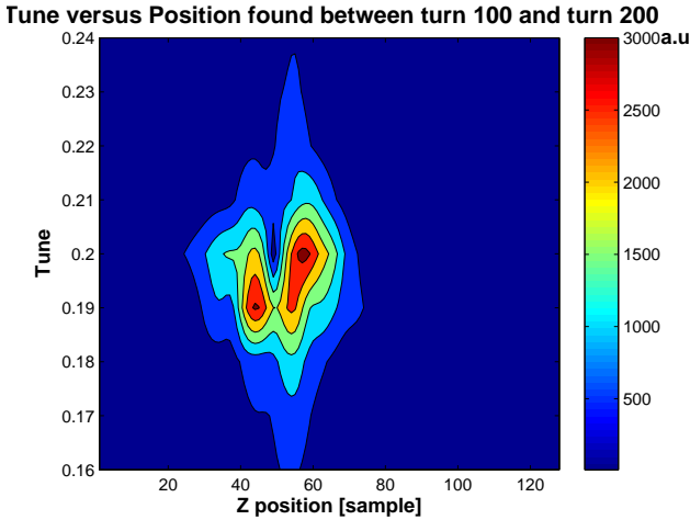
Figure 3: Tune vs. Z position, bunch 119, averaged over turns 100–200 after injection.
