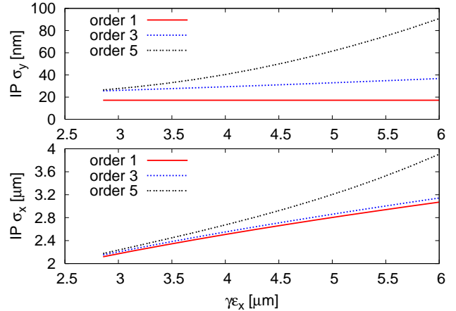
Figure 1: (top): Vertical beam size \sigma_y at the IP versus horizontal emittance for three different orders: first, third and fifth. Clearly the fifth order amplify dramatically the beam size. (bottom): Horizontal beam size \sigma_x at the IP versus horizontal emittance
