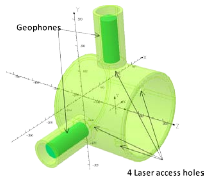
Figure 5: Magnetic shield design now has laser access to the magnetic center of the quadrupole coil. Four holes were created to maintain quad symmetry (only two used for lasers). Additional shielding around the Geophones counters local field spikes near the other penetrations.
