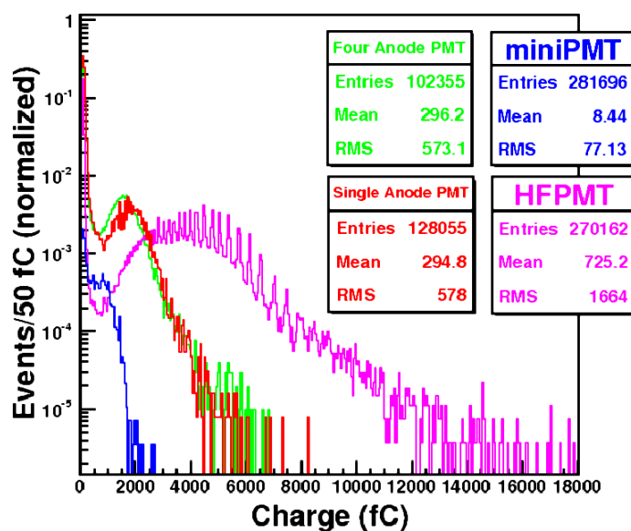
Figure 5. Charge distributions of the four anode PMT (R7600U-200-M4), the single anode PMT (R7600U-200), the miniPMT and the HFPMT produced by the front beam incidence.
