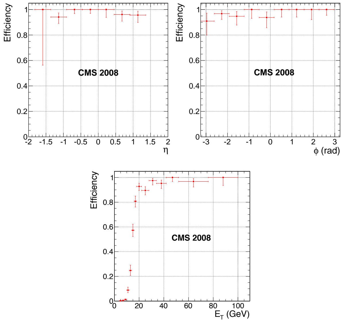
Figure 25: The efficiency of the single jet trigger with a L1 E_T threshold of 10 GeV, as a function of offline jet \eta , \phi , and E_T (with E_T > 25\text{GeV} for the \eta and \phi plots).
