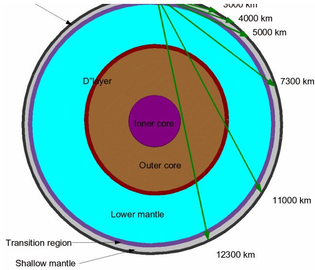
Figure 45. Several baselines projected through the model of the Earth interior (not to scale). A baseline of O(5000\text{ km}) may be problematic as it largely intersects with the transition zone, where the density changes quite abruptly from 4.0 to 4.4, and errors on its depth may result in large errors in the density profile. We see that the second and third magic baselines (11000 km and 12300 km) traverse through the outer core that dominates their refraction lengths.
