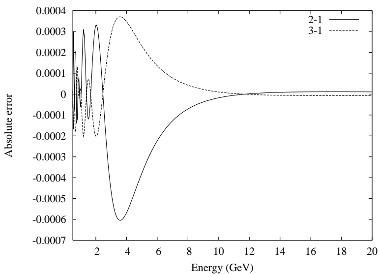
Figure 46. A sample plot presenting the effect of the uncertainties in the density profile of figure 44 to the muon neutrino appearance probability due to errors in density. These correspond to the absolute deviation in the probability with typical parameters.
