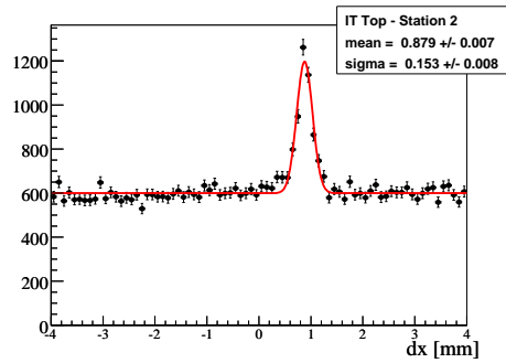
Figure 6: Pre-alignment: residuals in the Top box of IT-station T2.
