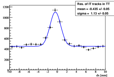
Figure 8: Residuals from IT tracks in TT.
