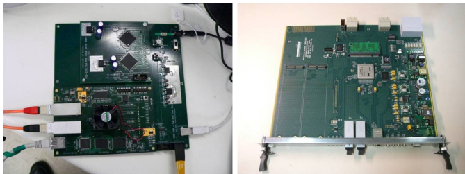
Figure 8: ROD injector board (left) and ROD prototype in ATCA format (right).
