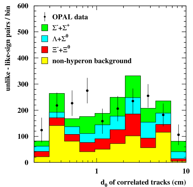
Fig. 5 Impact parameters of the displaced tracks, correlated to \Sigma^- candidates. The difference between unlike-sign and like-sign combinations is shown. Points: data. Histograms: results of the fit, ordered according to the sources for displaced tracks. The plotted errors are the statistical errors of the data
