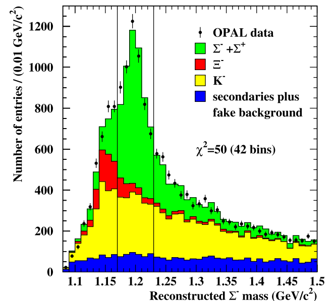
Fig. 3 Measured \Sigma^- mass spectrum. Points: data. Histograms: results of the fit, ordered according to the sources for track kinks. The plotted errors are the statistical errors of the data
