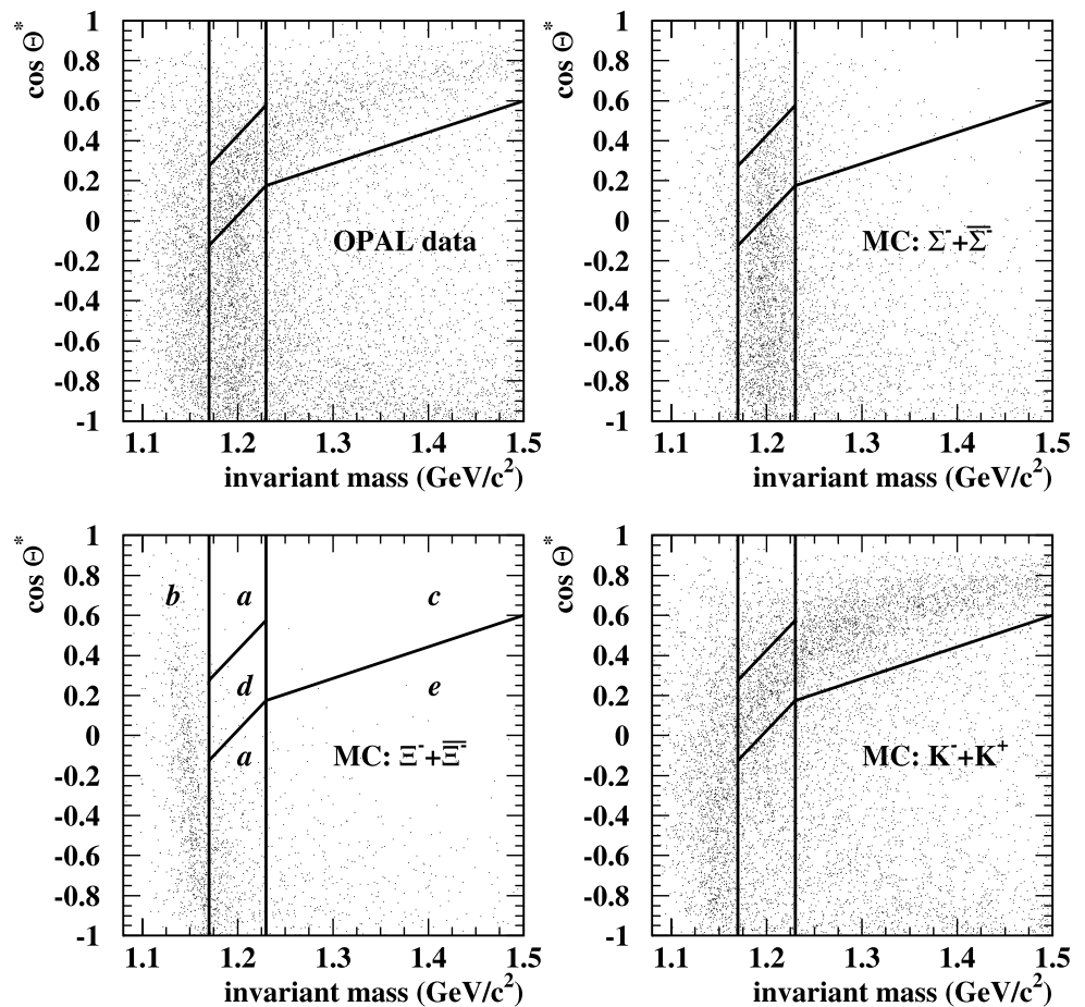
Fig. 2 Definition of two-dimensional bins to disentangle \Sigma^- hyperons from background. The reconstructed mass is plotted versus the pion emission angle in the hypothetical center-of-mass system. Top left : data. Other plots: Monte Carlo simulations for three particle classes as indicated. The labeling of the two-dimensional bins is shown in the bottom left plot. The preferential bins for the kink sources are: a + d for \Sigma^- and \bar{\Sigma}^+ , b for \Xi^- , b, c and d for K^- and e for background
