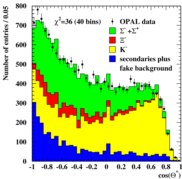
Fig. 4 Cosine of the center-of-mass pion emission angle. Points: data. Histograms: results of the fit, ordered according to the sources for track kinks. The plotted errors are the statistical errors of the data
