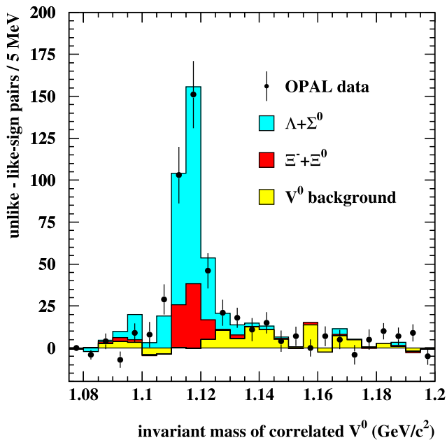
Fig. 7 Reconstructed masses of the \bar{\Lambda} candidates, correlated to \Sigma^- candidates. The difference between unlike-sign and like-sign combinations is shown. Points: data. Histograms: results of the fit, ordered according to the V^0 sources. The plotted errors are the statistical errors of the data
