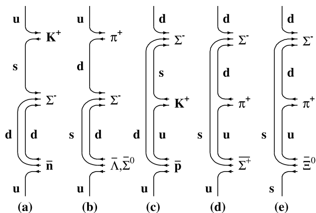
Fig. 1 Baryon production in the diquark model without (a, b) and with (c–e) the popcorn effect
