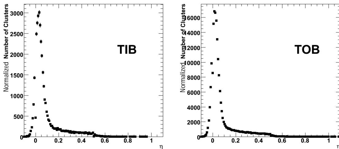
Figure 34. \eta function for TIB(left) and TOB(right) clusters. The data are from Virgin Raw runs where the information of the strips below the clustering threshold is available.
