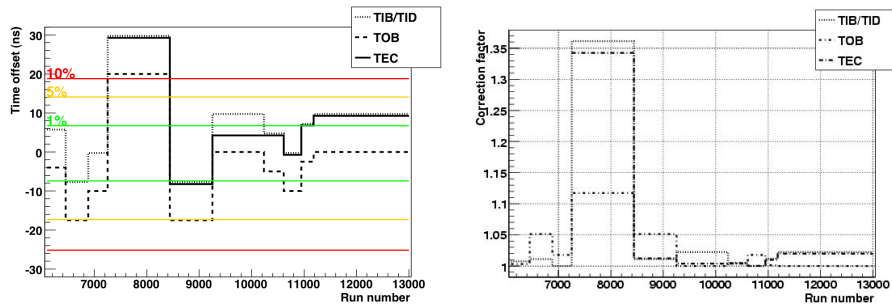
Figure 17. Offset from the on-peak timing (left) and signal correction factor (right) as function of the run number for the three sub-detectors TIB/TID, TOB, and TEC.
