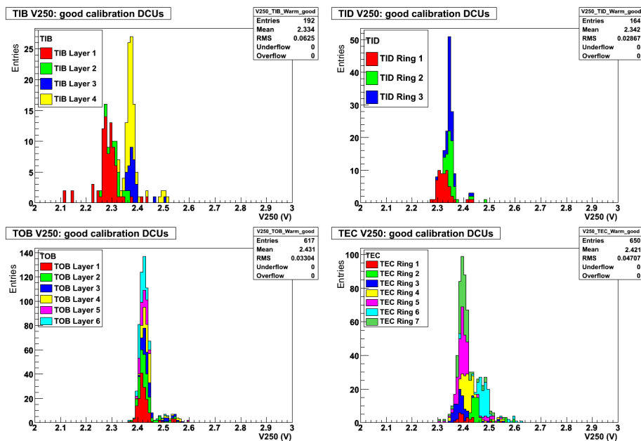
Figure 5. 2.5 V voltage line value measured at the module for TOB, TIB, TEC, and TID.
