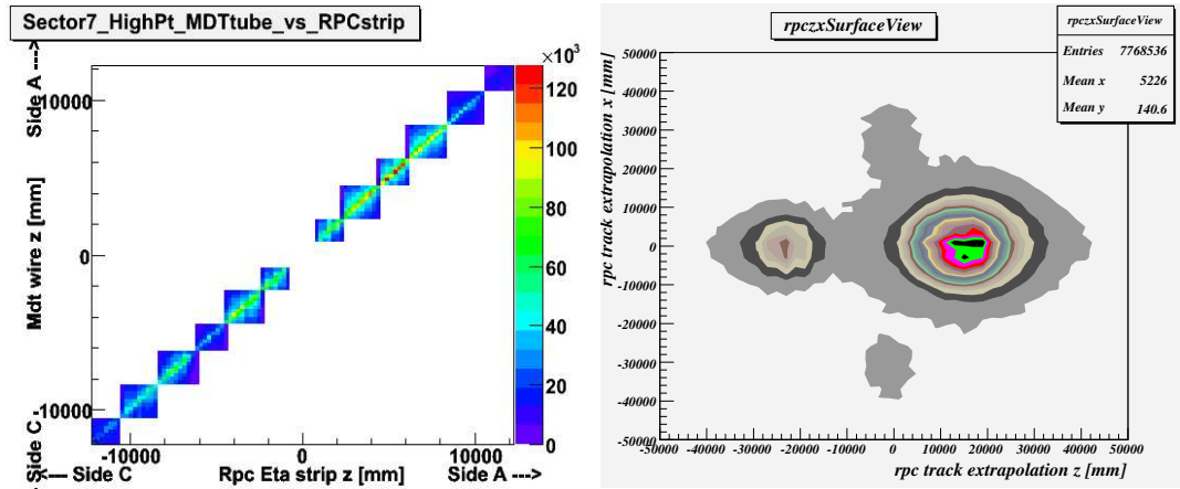
Figure 3: Hit spatial correlation along the beam (z axis) of adjacent MDT multi-layers and RPC planes (a). Extrapolation on surface of the cosmic muon triggered and reconstructed by the ATLAS RPC detector. In addition to the two main ATLAS shaft ( z=0 axis), the ATLAS service lifts are also clearly visible (b).
