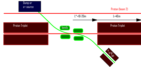
Figure 8: Schematic of linac-ring interaction region.
