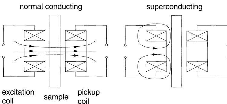
FIGURE 3 Schematic sketch of the susceptibility measurement. The external DC magnetic field is applied parallel to the sample surface.
