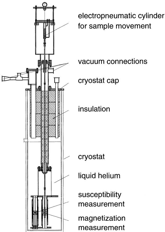
FIGURE 1 Cryostat with facilities for magnetization and susceptibility measurements at 4.2 K.
