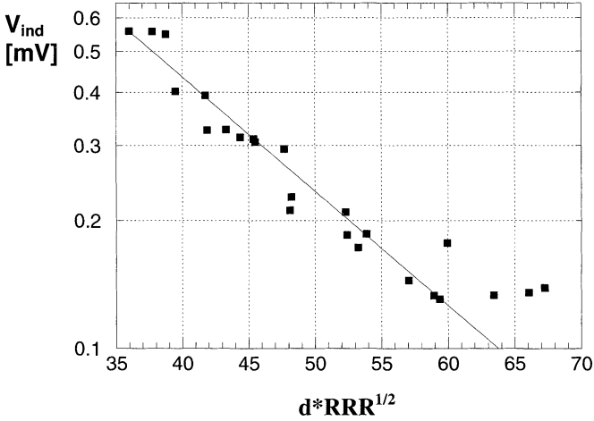
FIGURE 8 Step height observed in the susceptibility measurements of the transition from the superconducting to the normal conducting phase in dependence from the sample thickness d and the RRR value.
