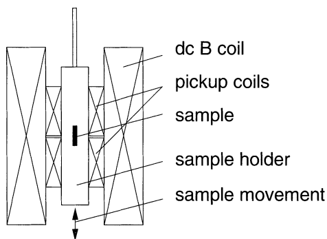
FIGURE 2 Schematic sketch of the magnetization measurement.
