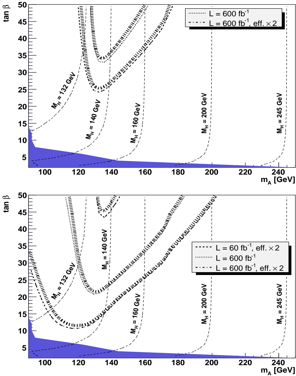
Figure 6. 5\sigma discovery contours (upper plot) and contours of 3\sigma statistical significance (lower plot) for the H \rightarrow \tau^+\tau^- channel in CEP in the M_A - \tan\beta plane of the MSSM within the M_h^{\max} benchmark scenario (with \mu = +200\text{GeV} ) for different luminosities. The values of the mass of the heavier CP-even Higgs boson, M_H , are indicated by contour lines. No pile-up background assumed. The dark shaded (blue) region corresponds to the parameter region that is excluded by the LEP Higgs boson searches.
