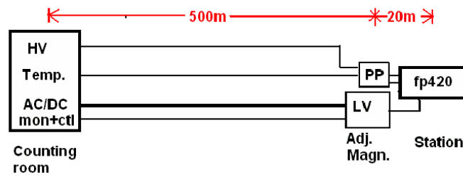
Figure 94. Overview of the Wiener Solution 1, with MPOD LV next to cryostat, MPOD HV in the counting room. “Station” indicates the FP420 cryostat and “Adj. Magn.” the magnets adjacent to the FP420 cryostat. “PP” is a patch panel.
