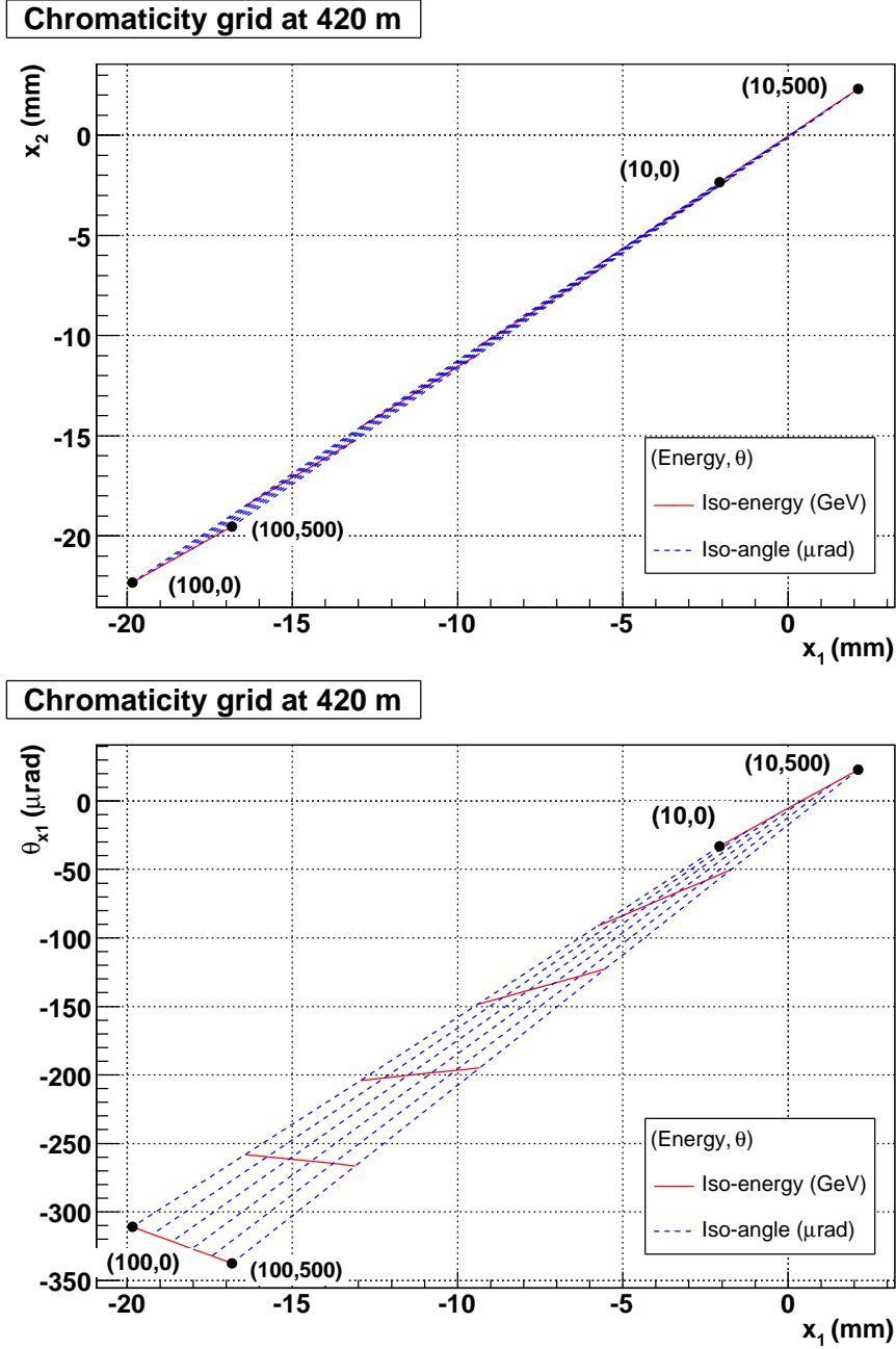
Figure 124. Chromaticity grids: iso-energy loss and iso-production angle lines, from 10 GeV to 100 GeV and 0 to 500 \mu\text{rad} [61].
