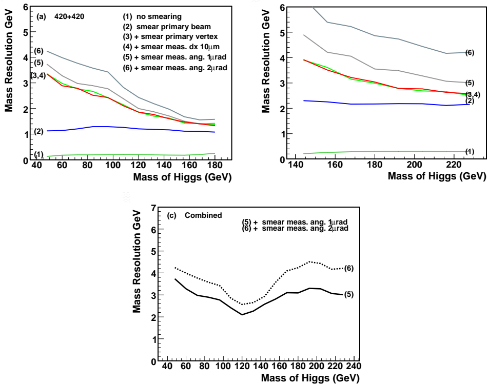
Figure 32. Mass resolutions obtainable in ATLAS (a) for 420 + 420 m measurements, (b) for 420+220 m measurements, (c) combined. The curves have different amounts of smearing applied as explained in the text.
