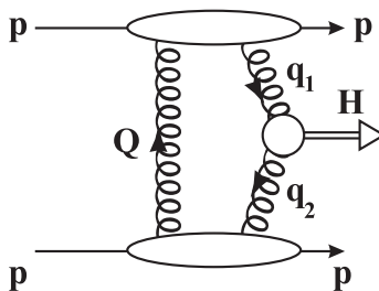
Figure 1. Central Exclusive Production (CEP): pp \rightarrow p + H + p .
