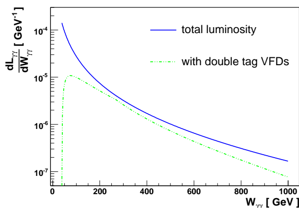
Figure 8. Relative elastic luminosity spectrum of photon-photon collisions at the LHC in the range Q_{\min}^2 < Q^2 < 2 \text{ GeV}^2 (solid blue line) compared to the corresponding luminosity if the energy of each photon is restricted to the forward detector (VFD) tagging range 20 \text{ GeV} < E_\gamma < 900 \text{ GeV} (dashed green curve) [12].
