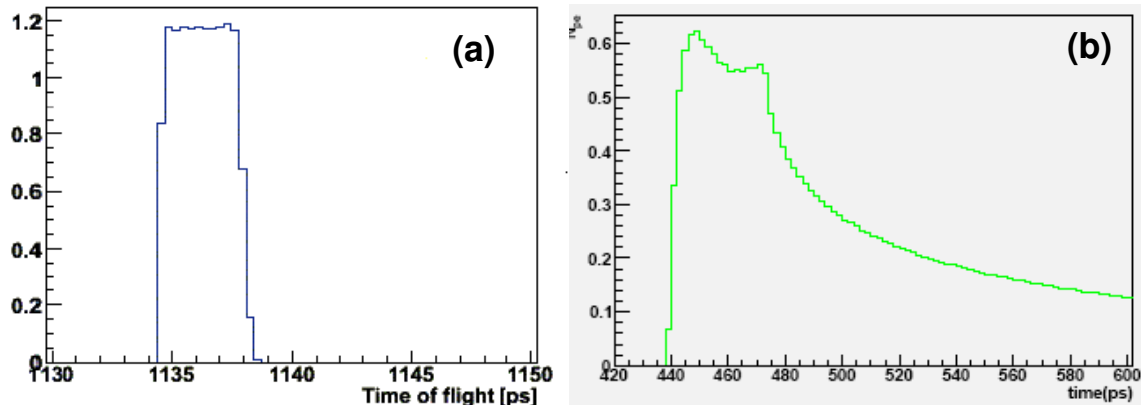
Figure 116. Simulated time of arrival of Čerenkov photons at the MCP-PMT photocathode for (a) GASTOF (b) QUARTIC.
