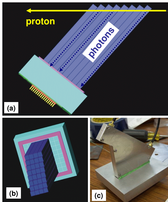
Figure 115. Conceptual drawings of a QUARTIC detector, (a) showing the proton passing through eight bars of one row in x providing eight measurements of the proton time (b) showing the 4 \times 8 layout of QUARTIC bars (c) A photograph of the prototype detector used in the June 2008 CERN test beam.
