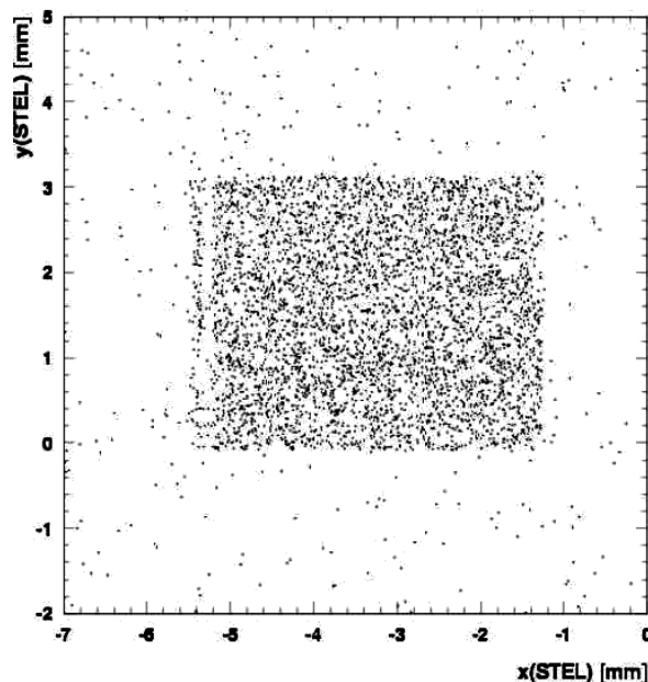
Figure 66. Two-dimensional efficiency map of a fully operational 3D detector. A point is plotted with respect to the position (x, y) predicted by a telescope, with a precision of 4 \mu\text{m} as a valid track and a hit was recorded by a 3D detector. The inefficient band near the lower x -edge was caused by the detector’s bonding pads. The upper and lower y edges were used for active edge measurements and showed a device sensitivity up to 4 microns from the physical edge.
