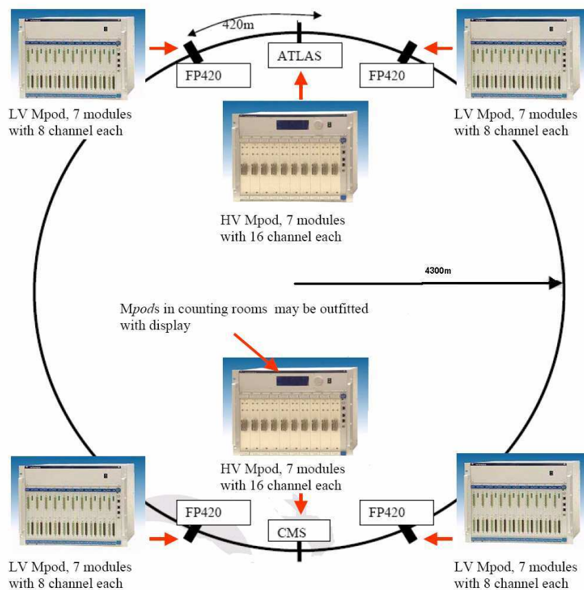
Figure 95. Wiener solution with LV supplies in the tunnel and HV supplies in the counting room, delivering the bias via 500 m cables. The MPOD will require custom –120 V modules.
