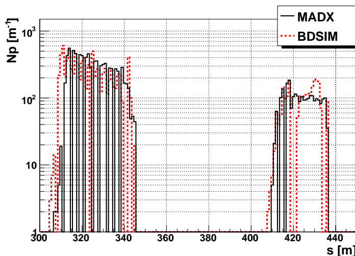
Figure 43. Loss maps produced for the IP5 beamline with a DPMJET phase space sample using MADX and BDSIM.
