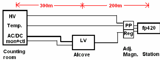
Figure 98. Low voltage in alcoves, rest in counting room using 200 m cables from alcove to cryostat. “Station” indicates the FP420 cryostat and “Adj. Magn.” the magnets adjacent to the FP420 cryostat. “PP” is a patch panel. “Reg” are linear regulators next to the load.
