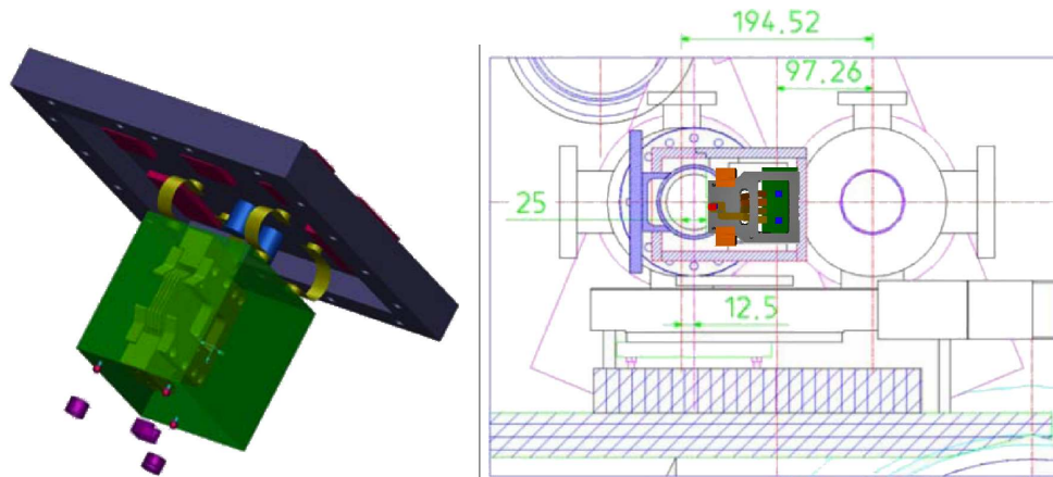
Figure 88. Left: A complete tracking station attached to the lid. Also shown are the positioning studs. Right: Schematic view of the box in position around the beam pipe.
