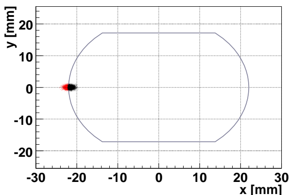
Figure 25. Example of aperture check for a typical Main Bending dipole at 338m from IP5, for a set of protons with a mean energy loss of 110 GeV. The protons which exit the aperture are shown in black, and those which hit the walls are shown in red.
