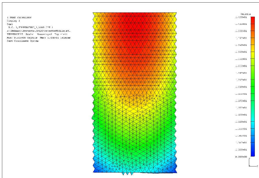
Figure 107. Gradient in the CE7 plane underneath the tracker cell (4.3°C).
