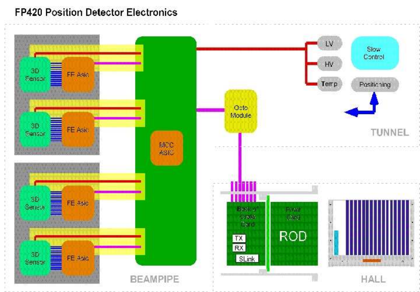
Figure 102. Layout of the readout and DAQ system.
