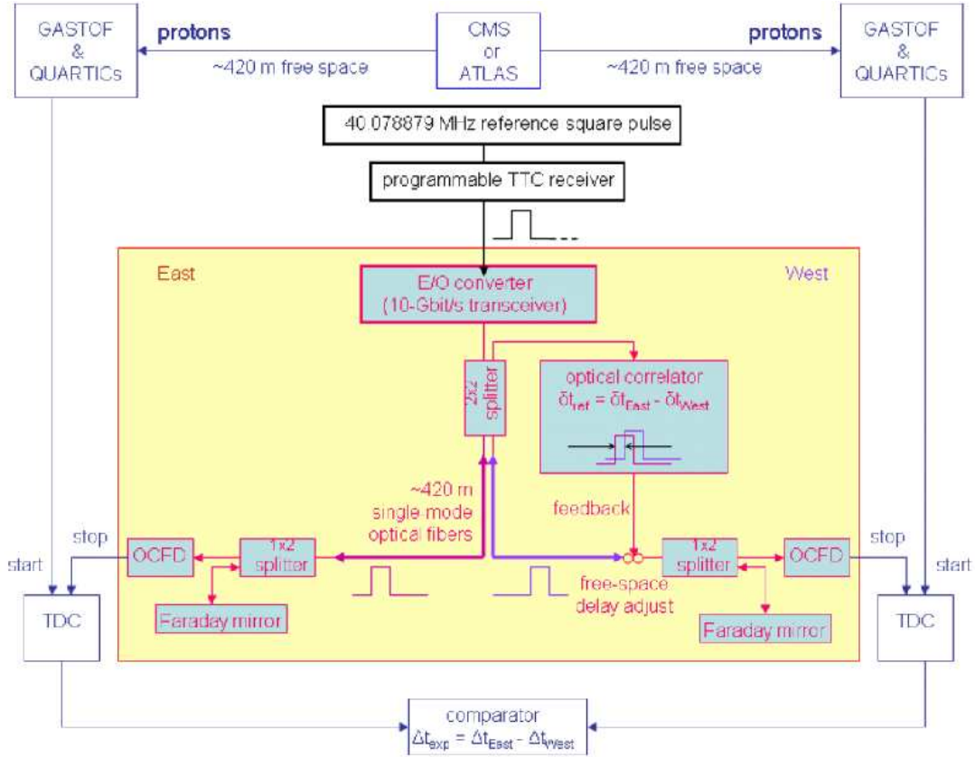
Figure 119. A schematic of the reference time system. Components labeled in black are expected to come from CERN TTC system, components labeled in blue are associated with the ToF detectors, and the components in red (highlighted in the yellow box) are the optical components related to the reference timing system.
