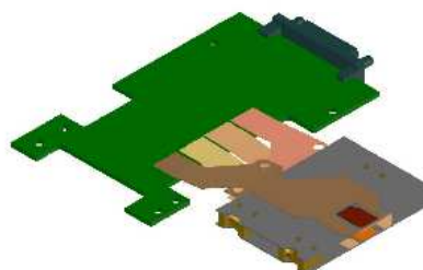
6. Flex connections bonded to the MCC PCB
