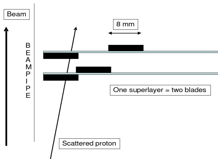
Figure 80. Schematic of a superlayer consisting of four sensors.
