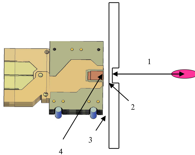
Figure 89. Key dimensions from the beam to the edge of the first chip. 1 — beam to window, 2 — window thickness, 3 — standoff of detector from window depends on thermal considerations and assembly tolerances, 4 — distance of first pixel from from edge of blade defined by dicing considerations.
