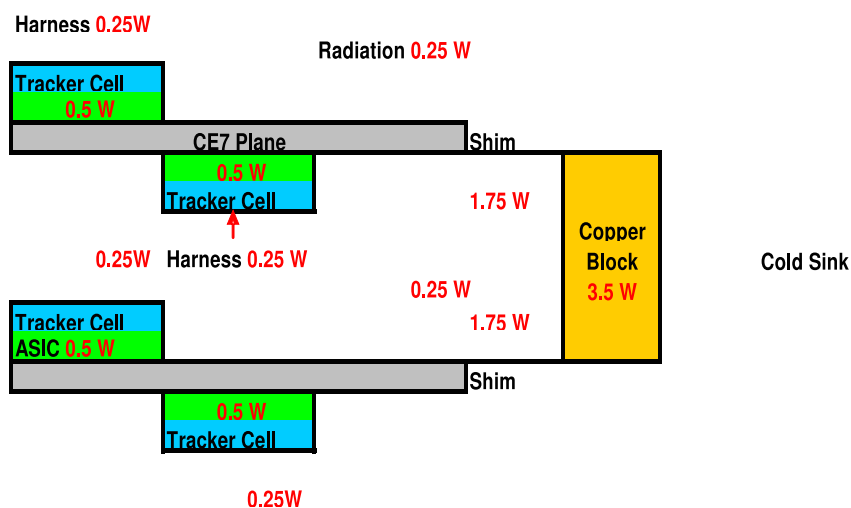
Figure 105. Heat flow surrounding the tracker cells (local thermal network).
