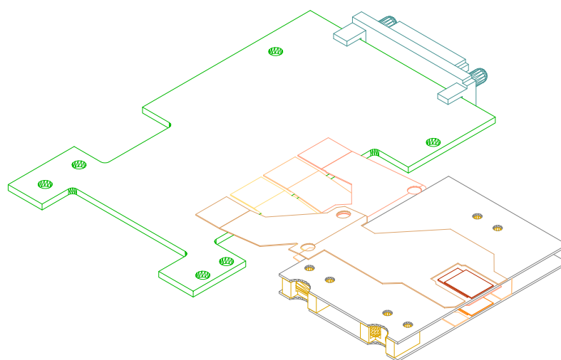
Figure 81. A schematic drawing of a superlayer, consisting of two blades. The flexible circuits connect the four sensors to a common control card.
