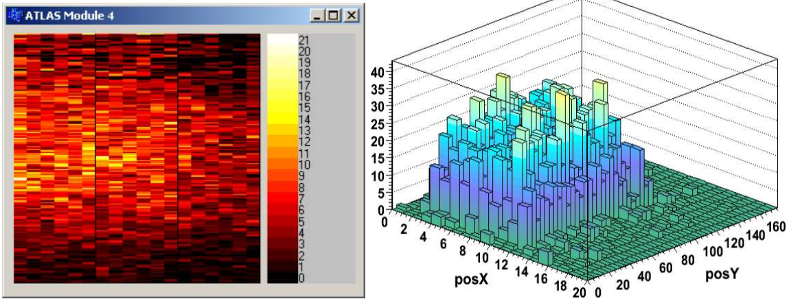
Figure 72. Hit map for a 12 \times 12 \text{ mm}^2 (left) and lego-plot for a 3 \times 3 \text{ mm}^2 (right) scintillator trigger. Device 3D-2E-A operated at 30 V.
