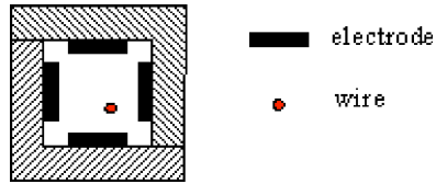
Figure 121. A cross-sectional schematic of a WPS sensor and alignment wire.
