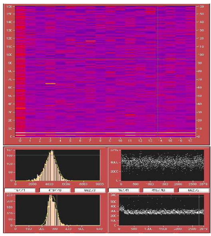
Figure 76. Snapshot of the online display of the TurboDaq ATLAS pixel test setup. On the top the entire pixel matrix response to a test pulse. At the bottom the ENC (Equivalent Noise Charge) is measured as the sigma of the threshold distribution.
