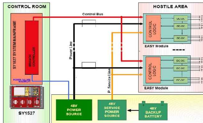
Figure 92. Block diagram of the CAEN setup.
