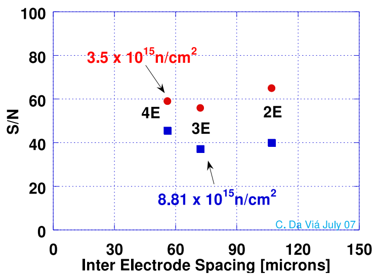
Figure 78. Extrapolated Signal to Noise (S/N) ratios of three 3D pixel configurations at two different irradiation fluences.
