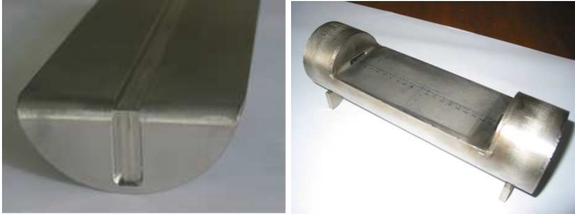
Figure 53. Hamburg pipe prototypes: (left) an end view of a machined window before welding to the beam-pipe; (right) a 200 mm long pocket, TIG welded in a tube without reinforcement.
