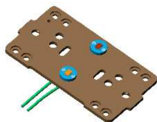
3. Chips transferred and held by vacuum
