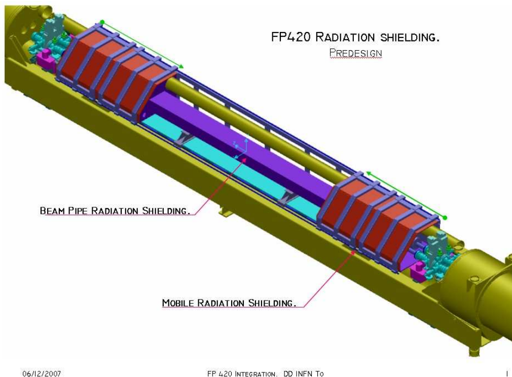
Figure 48. Preliminary design for radiation shielding around the warm beampipes and detector stations. The mobile shielding can be rolled sideways on rails to give access to the detector stations.
