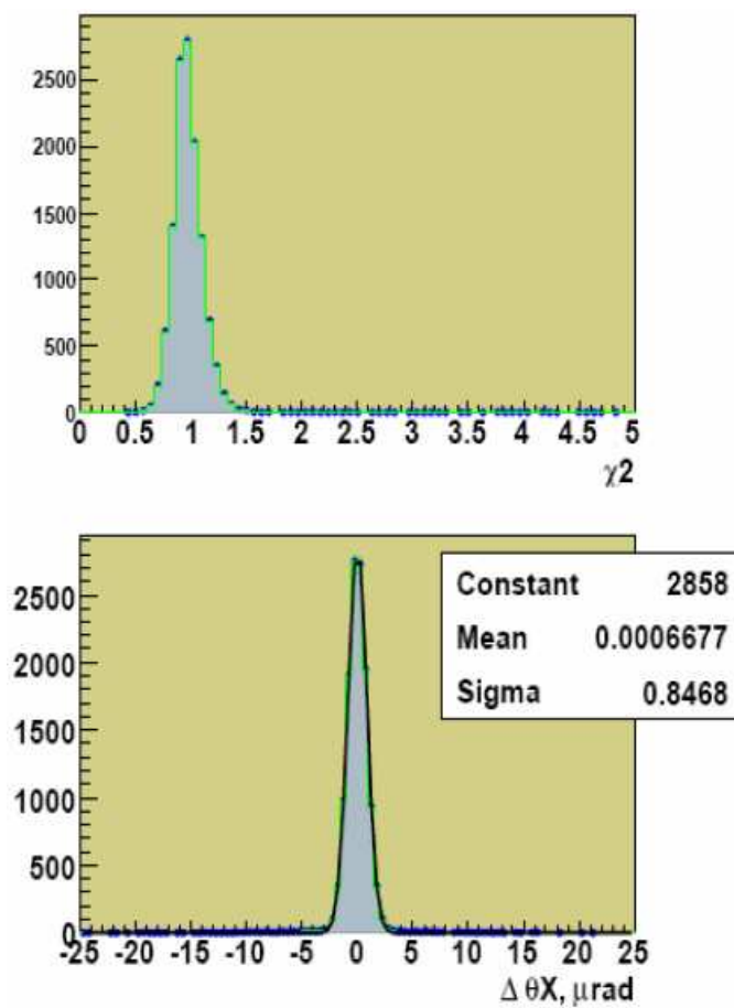
Figure 111. Track \chi^2/\text{NDF} (top) and angular resolution (bottom) for a two-station tracker. The angular resolution is 0.85 \mu\text{rad} if the \chi^2/\text{NDF} is selected to be less than 1.5.
