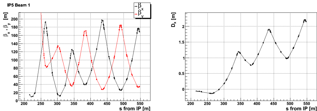
Figure 33. The betatron functions and horizontal dispersion in the FP420 region for Beam 1 downstream of IP5.
