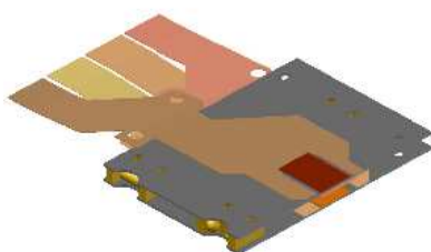
5. Blades A&B assembled to form a superplane
