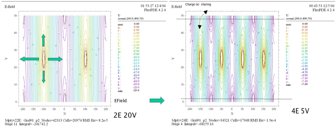
Figure 70. Equipotentials in a 2E and 4E 3D detector. Pixel size is 50\ \mu\text{m} (Y) by 400\ \mu\text{m} (X). The bias is 20 V and 5 V for the 2E and 4E devices respectively. The direction of the electric field is indicated. The n-electrodes are at the centre. A maximum field of 1\ \text{V}/\mu\text{m} occurs at 24 V and 14 V in a 2E and 4E device respectively.
