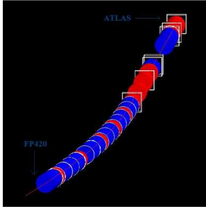
Figure 41. Beam line model created with BDSIM, showing the beamline from ATLAS to the position of the FP420 detector (red denotes a quadrupole element and blue denotes a bending element).
