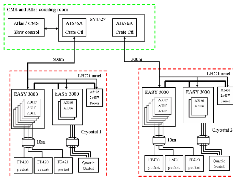
Figure 93. Diagram of the solution suggested by CAEN. The number of pockets assumed is 3 per cryostat. Shown are also the system for temperature monitoring (A3801) and the supplies for QUARTIC/GASTOF detectors (A3540 and A3006).
