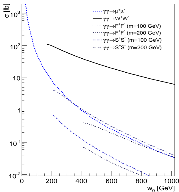
Figure 9. Cross sections for various \gamma\gamma processes at the LHC as a function of the minimal \gamma\gamma centre-of-mass energy W_0 [12].
