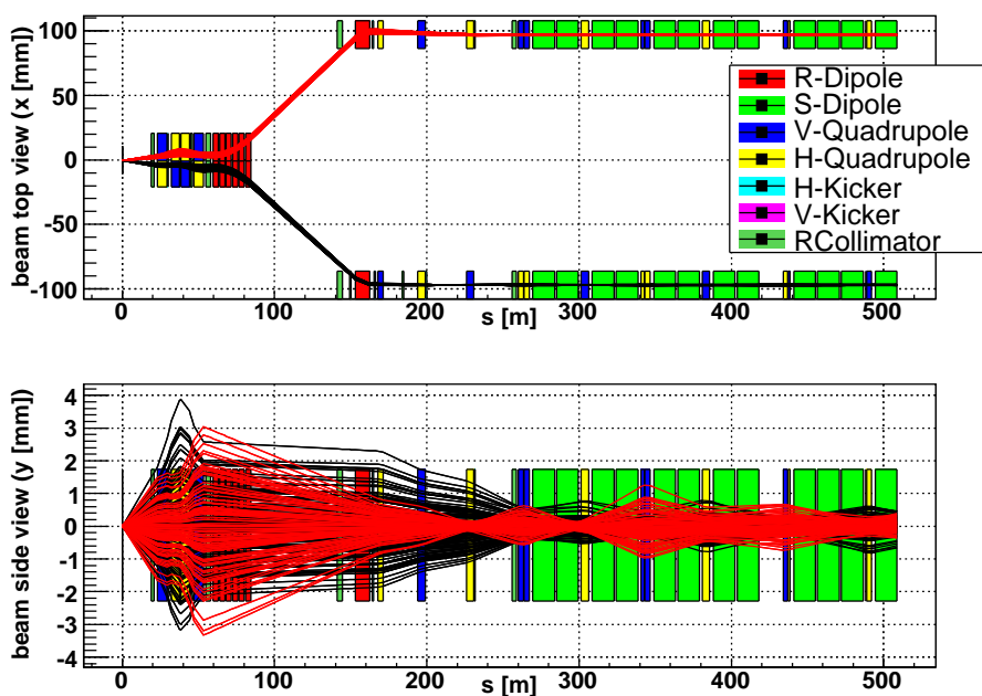
Figure 23. Schematic plan view and side view of the beamline at IP5 (CMS); the IP1 configuration (ATLAS) is similar except that the kicker magnets are vertical (see also figure 123) [61]. The horizontal curvature of the beamline has been straightened out for purposes of simplification here.
