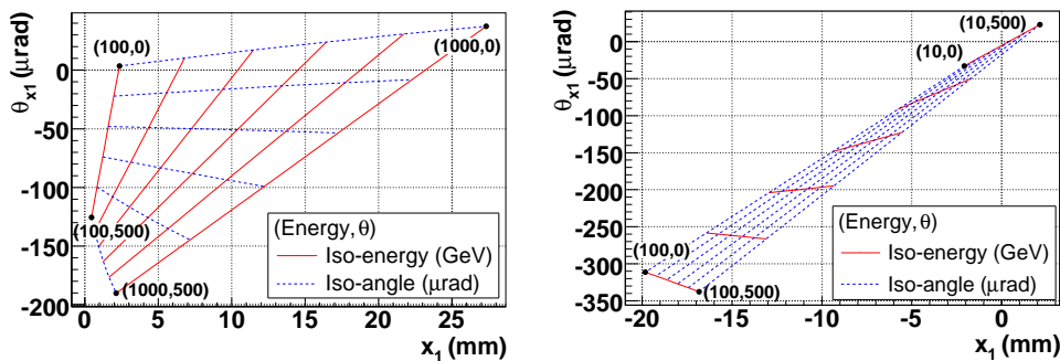
Figure 27. Chromaticity grids: iso-energy and iso-angle lines for 220 m (left) and 420 m (right) detectors at IP5, beam 1 computed with HECTOR. The vertical axis \theta_{x1} is the angle of the scattered proton relative to the beam at 220 or 420 m, and the horizontal axis x_1 is the horizontal displacement of the scattered proton relative to the beam. The solid red lines are iso-energy lines, ranging from proton energy loss 0 GeV to 1000 GeV in steps of 200 GeV at 220 m, and from 0 GeV to 100 GeV in steps of 20 GeV at 420 m. The dotted blue lines are lines of constant proton emission angle at the interaction point, and range from 0 \mu\text{rad} to 500 \mu\text{rad} in steps of 100 \mu\text{rad} .
