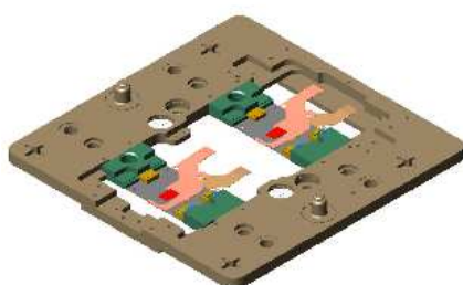
3. Two Blade B's inserted in turnplate aligned by small touch bearings
