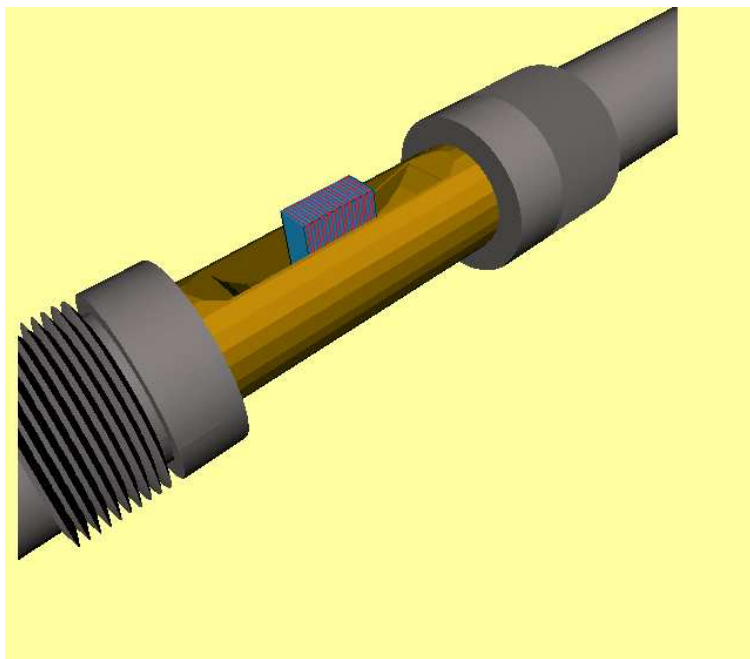
Figure 45. An example of the GEANT 4 geometry of the pocket hosting the detectors. This model was used to study the interaction rate of 7 TeV protons, which is described in section 9.7.
