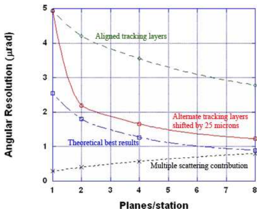
Figure 108. Angular resolution for a tracker consisting of two stations separated by 8 metres. Each layer has a detector with a pitch of 50 microns. The curves from top to bottom are: aligned tracking layers, alternate layers shifted by 25 microns, theoretical best result, and multiple scattering contribution. The design goal is one \mu\text{rad} .
