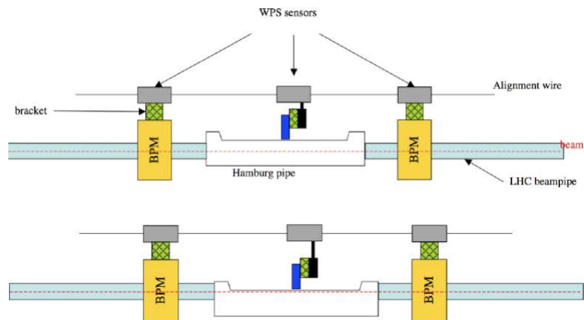
Figure 120. The proposed overall alignment system, shown with detectors in garage position (top picture) and in operating position (bottom picture).
