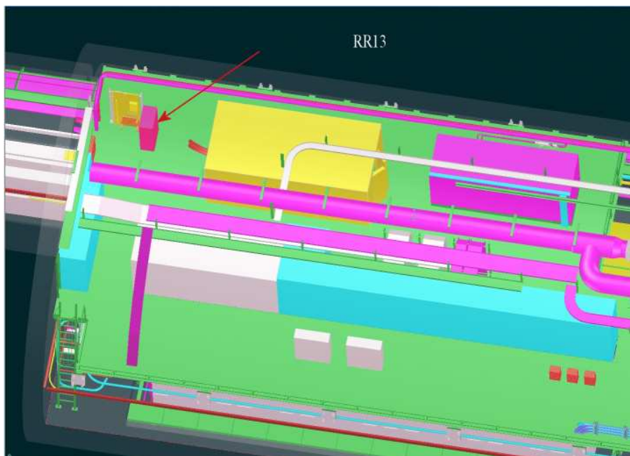
Figure 127. Reserved rack space in the LHC alcove areas (RRs).
