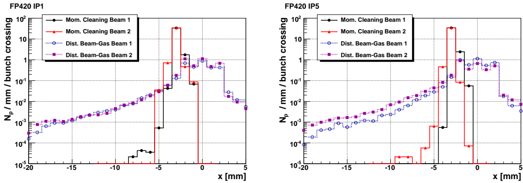
Figure 38. Horizontal distribution of the protons emerging from the momentum cleaning collimators and scattered due to beam-gas interaction, as observed at 420 m, after normalization for the beam lifetime as described in text.
