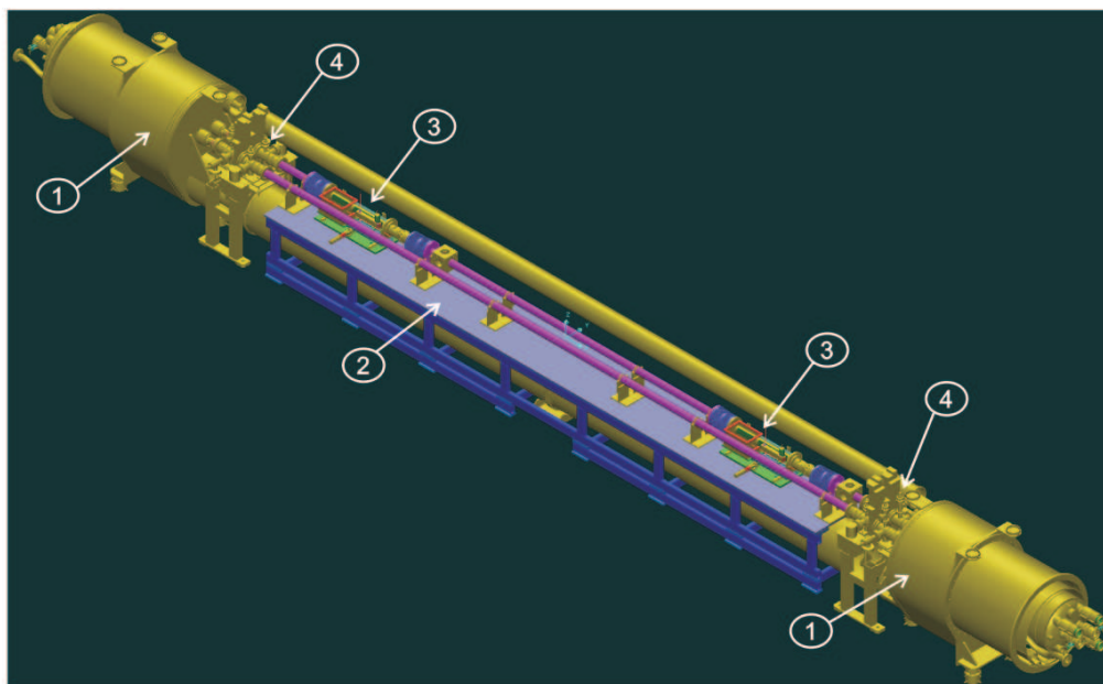
Figure 49. Schematic view of the connection cryostat (1) and detector arm with support table (2), two detector sections (3) and vacuum pumping sections (4).
