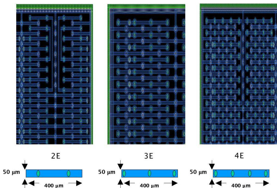
Figure 69. Different 3D cell structures designed to be compatible with the ATLAS Pixel detector readout chip. The pixel size is 50 μm by 400 μm. The devices have either 2, 3 or 4 electrodes per pixel and are named 2E, 3E and 4E respectively. The electrodes cover 4%, 6% and 8% of the total area for 2E, 3E and 4E devices respectively.
