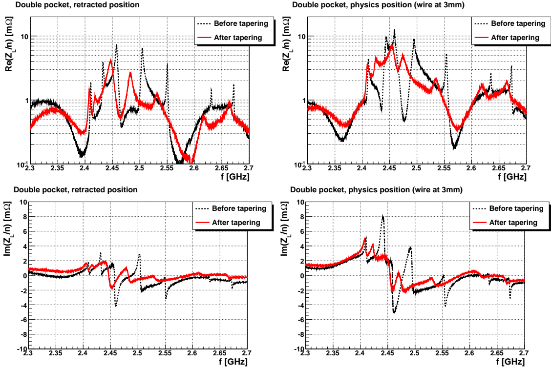
Figure 62. Real and imaginary part of the longitudinal impedance for the FP420 physics (inserted) and parking positions, as measured for a double pocket prototype.
