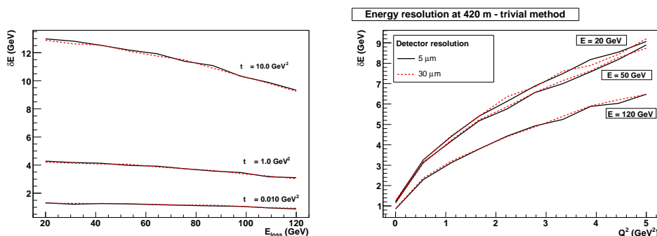
Figure 31. Energy resolution for the simple reconstruction method described in the text for protons at 420 m. The resolution is shown as a function of energy loss (left) and Q^2 (= -t) (right). Also shown is the effect of varying the error on the positional measurement on the detectors from 5 \mu\text{m} to 30 \mu\text{m} .
