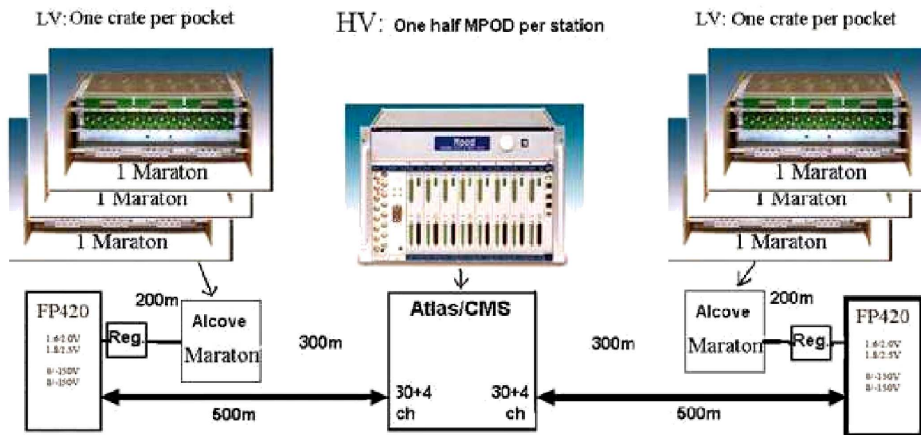
Figure 99. Low-voltage Wiener Maraton supplies in the alcoves. High-voltage MPOD supplies in the counting room. The Wiener Maraton system is qualified for the expected radiation environment within a large margin. “Station” indicates cryostat.
