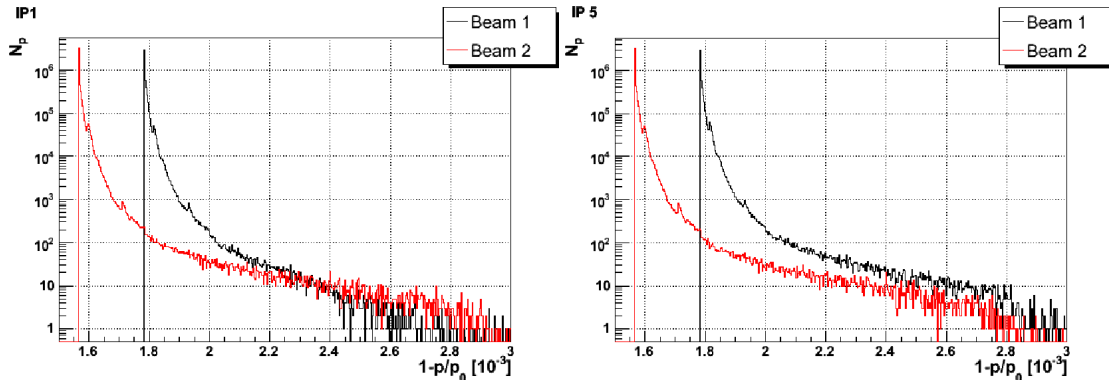
Figure 35. Momentum distribution of the protons emerging from the momentum cleaning collimators.
