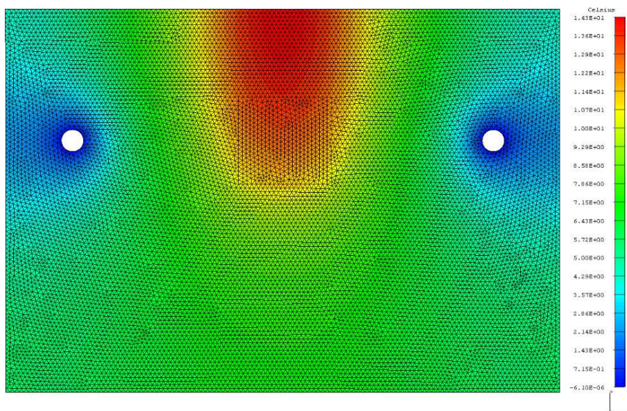
Figure 106. CE7 detector plane gradient (worst-case configuration).
