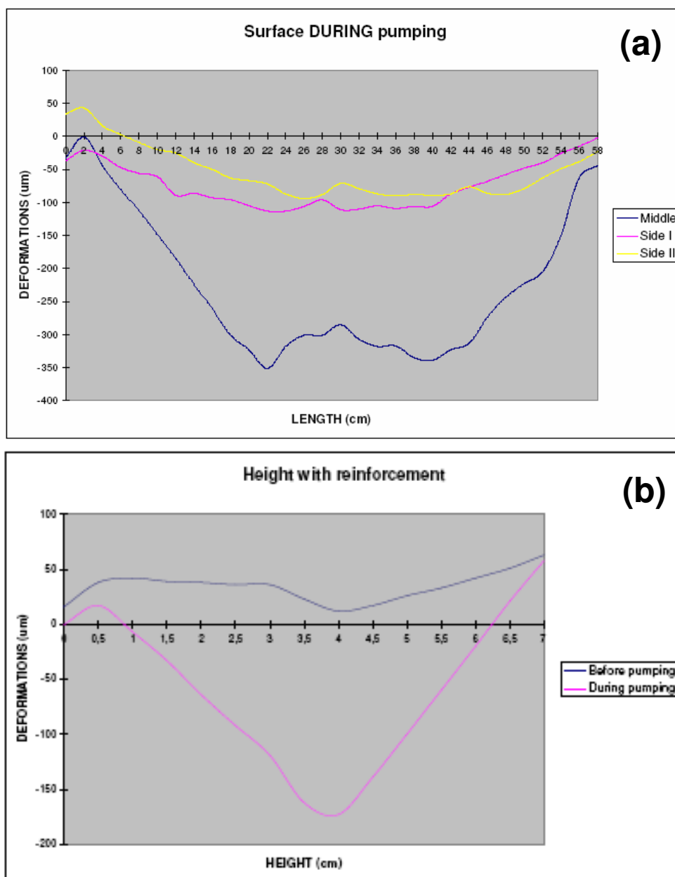
Figure 56. (a) Deformation as a function of length after vacuum pumping. (b) Height profiles after reinforcement.
