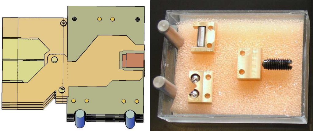
Figure 86. Left: Several superplanes showing the bearings without the support structure. Right: Miniature touch bearing. The ball bearings are 3mm diameter.
