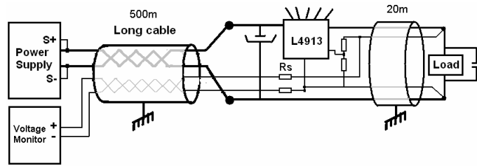
Figure 90. Block diagram showing the principle of using a local radiation-hard linear regulator. Here for a positive voltage and the option of remote monitor of the load voltage via isolation resistors R_s .
