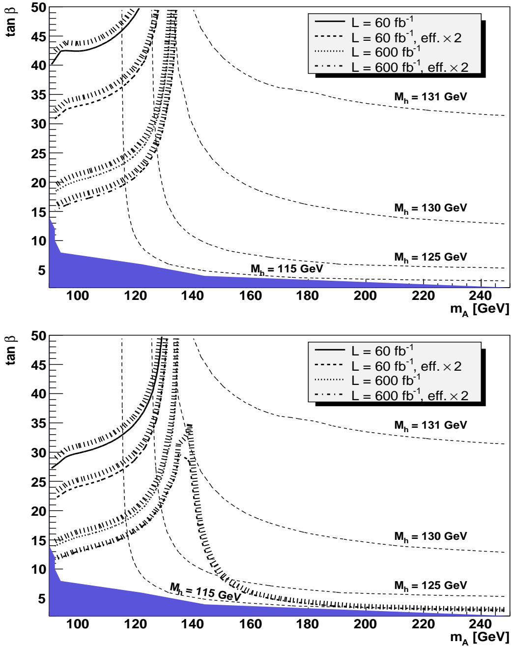
Figure 4. 5\sigma discovery contours (upper plot) and contours of 3\sigma statistical significance (lower plot) for the h \rightarrow b\bar{b} channel in CEP in the M_A - \tan\beta plane of the MSSM within the M_h^{\text{max}} benchmark scenario for different luminosity scenarios as described in the text [19]. The values of the mass of the light CP-even Higgs boson, M_h , are indicated by contour lines. No pile-up background assumed. The dark shaded (blue) region corresponds to the parameter region that is excluded by the LEP Higgs boson searches [42, 43].
