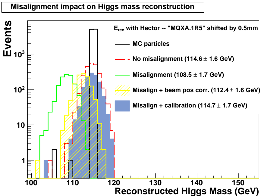
Figure 125. Illustration of the effect on the missing mass reconstruction due to a misalignment of LHC quadrupoles. In this example a quadrupole (MQXA1R5) has been misaligned by 500 \mu\text{m} . Data from BPMs cannot fully recover the mass shift, while the exclusive dimuon calibration recovers it fully, and the resolution is not affected as long as the misalignment is stable [61].
