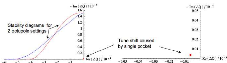
Figure 64. Tune shift induced by FP420 single pocket at 3 mm, due to resistive wall transverse impedance (calculations based on B. Zotter and E. Metral’s models). The effect is negligible when compared to the stability diagram that assesses how the LHC octupoles tuning can damp the instability.
