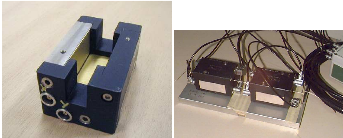
Figure 122. A WPS sensor with lid removed (left), showing the electrodes. The aperture is 1cm square. Also shown are two WPS sensors on the test bench (right).
