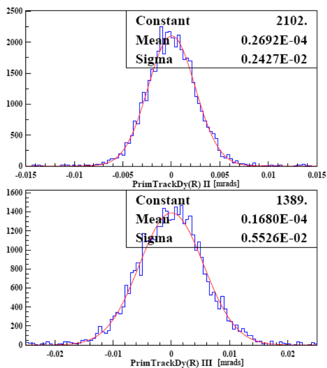
Figure 110. GEANT4 estimate of the multiple scattering (in mrad) in the middle (top) and at the end (bottom) of the three-station tracker.
