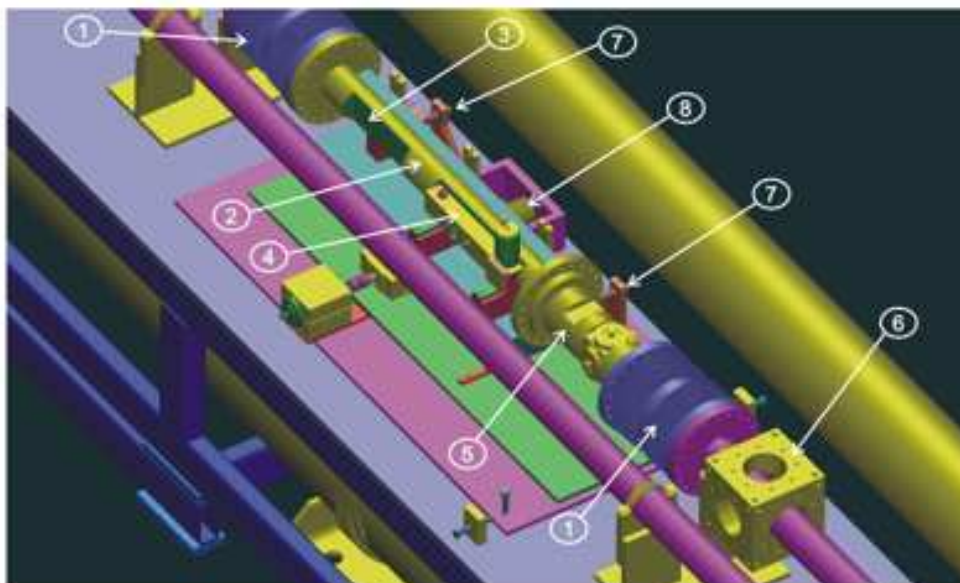
Figure 50. Top view of one detector section: bellows (1), moving pipe (2), Si-detector pocket (3), timing detector (4), moving BPM (5), fixed BPM (6), LVDT position measurement system (7), emergency spring system (8).
