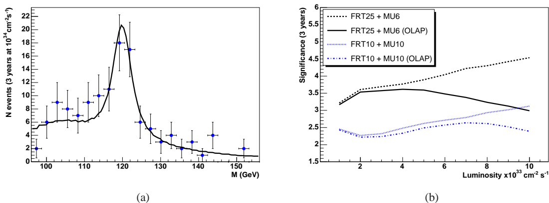
Figure 21. (a) Typical mass fit for the 120 \text{ GeV}/c^2 MSSM h \rightarrow b\bar{b} for 3 years of data taking at 10^{34} \text{ cm}^{-2} \text{ s}^{-1} after removing the overlap background contribution completely with improved timing detectors. The significance is 5\sigma for these data. (b) Significance of the measurement of the 120 \text{ GeV}/c^2 MSSM Higgs boson versus luminosity, for two different combinations of muon — MU6, MU10 — and jet-rate — FRT25, FRT10 — triggers, see section 3.1, and with an improved (baseline) FP420 timing design (OLAP labels).
