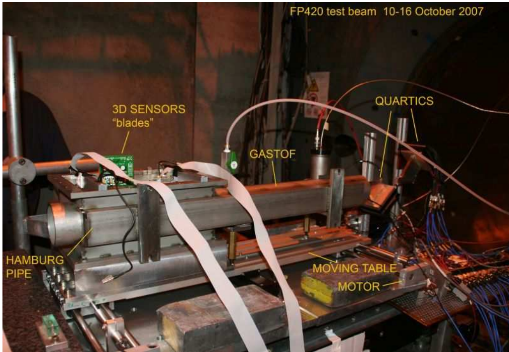
Figure 58. Photograph of the prototype beam-pipe section used in the October 2007 CERN test beam.
