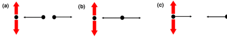
Figure 113. A schematic diagram of overlap backgrounds to central exclusive production: (a) [p][X][p] : three interactions, one with a central system, and two with opposite direction single diffractive protons (b) [pp][X] : two interactions, one with a central system, and the second with two opposite direction protons (c) [p][pX] : two interactions, one with a central system and a proton, the second with a proton in the opposite direction.
