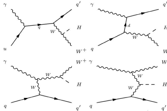
Figure 13. The Feynman diagrams for \gamma q \rightarrow HW^+q' associated production at LO [12].
