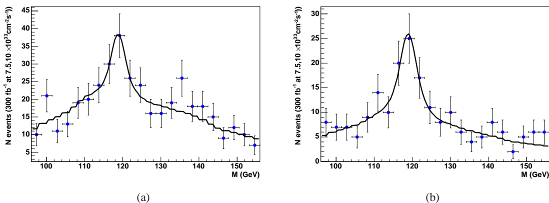
Figure 22. Mass fit for 300 \text{ fb}^{-1} of data for the improved background estimates described in the text (reduced CEP backgrounds, negligible [pp][X] and a luminosity profile consisting of half the data collected at 7.5 \times 10^{33} \text{ cm}^{-2} \text{ s}^{-1} and half at 10^{34} \text{ cm}^{-2} \text{ s}^{-1} ). The plots are made assuming (a) baseline timing of 10ps and (b) improved timing of 5 ps or central timing.
