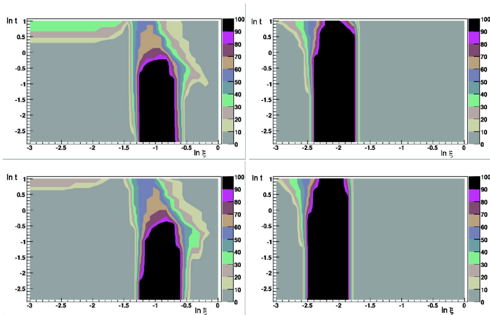
Figure 26. Acceptances in the \xi, t plane for protons to reach planes at 220 m (left) and 420 m (right) for beam-1 (top) and beam-2 (bottom) around IP1 (ATLAS) computed with FPTrack. The variables plotted are t , the modulus of the squared momentum transfer to the proton at the IP, and \xi , its fractional energy loss. No detector effects are included here.
