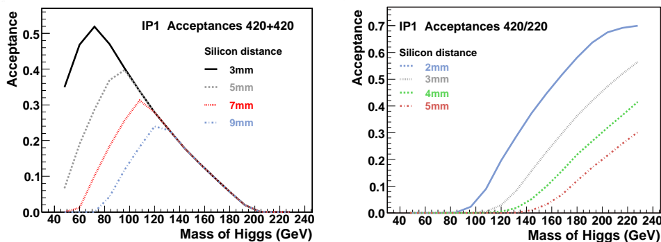
Figure 28. Acceptance as a function of centrally produced mass for (left) 420 + 420 m proton tags for the silicon detector active edge positioned at different distances from the beam; (right) for 220 + 420 m proton tags with the 420 m silicon at 5 mm from the beam and the 220 m at different distances from the beam. The small upward deviation at high mass for the 2 mm silicon positions, show the additional acceptance from 220 + 220 m coincidences.
