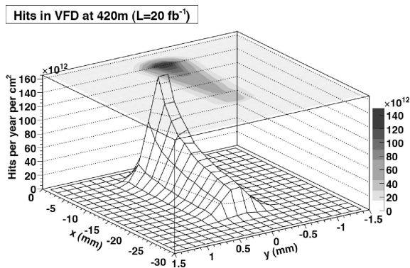
Figure 30. Number of proton hits due to the process pp \rightarrow pX for 20 \text{ fb}^{-1} integrated luminosity. Protons were generated with PYTHIA 6.2.10 (single diffraction process 93) and tracked through the beam lattice with HECTOR.
