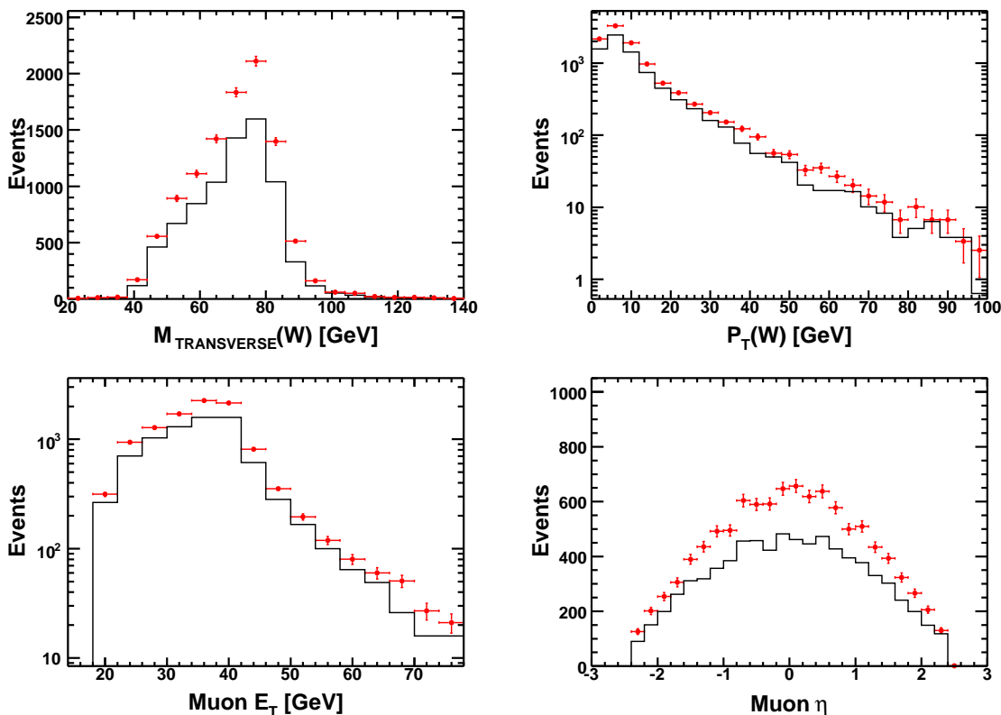
Figure 17. Distributions, for \int \mathcal{L} dt = 1 \text{ fb}^{-1} , of (a) transverse mass of the W^\pm boson, (b) transverse momentum of the W^\pm , (c) transverse momentum of the muon, (d) pseudorapidity of the muon for W \rightarrow \mu\nu . Full points: approximately flat diffractive gluon density (H1 fit 2 [89]); histograms: more peaked diffractive gluon density (H1 fit 3 [89]). From [8].
