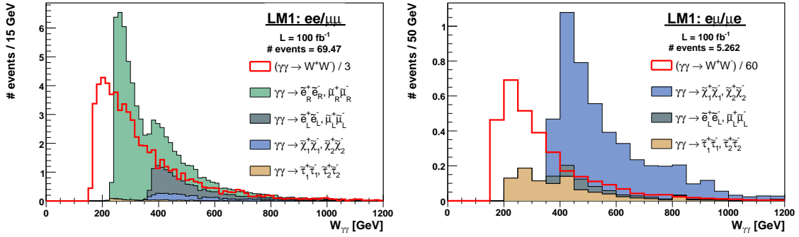
Figure 11. Photon-photon invariant mass for benchmark point LM1 with \int \mathcal{L} dt = 100 \text{ fb}^{-1} . Cumulative distributions for signal with two detected leptons ( p_T > 3 \text{ GeV}/c , |\eta| < 2.5 ), two detected protons, with same (left) or different flavour (right). The WW background has been down-scaled by the quoted factor [12].
