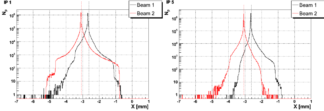
Figure 36. Horizontal distribution of the protons emerging from the momentum cleaning collimators as observed at FP420 after the simulations of 2 \cdot 10^6 proton interactions with the primary momentum cleaning collimators.
