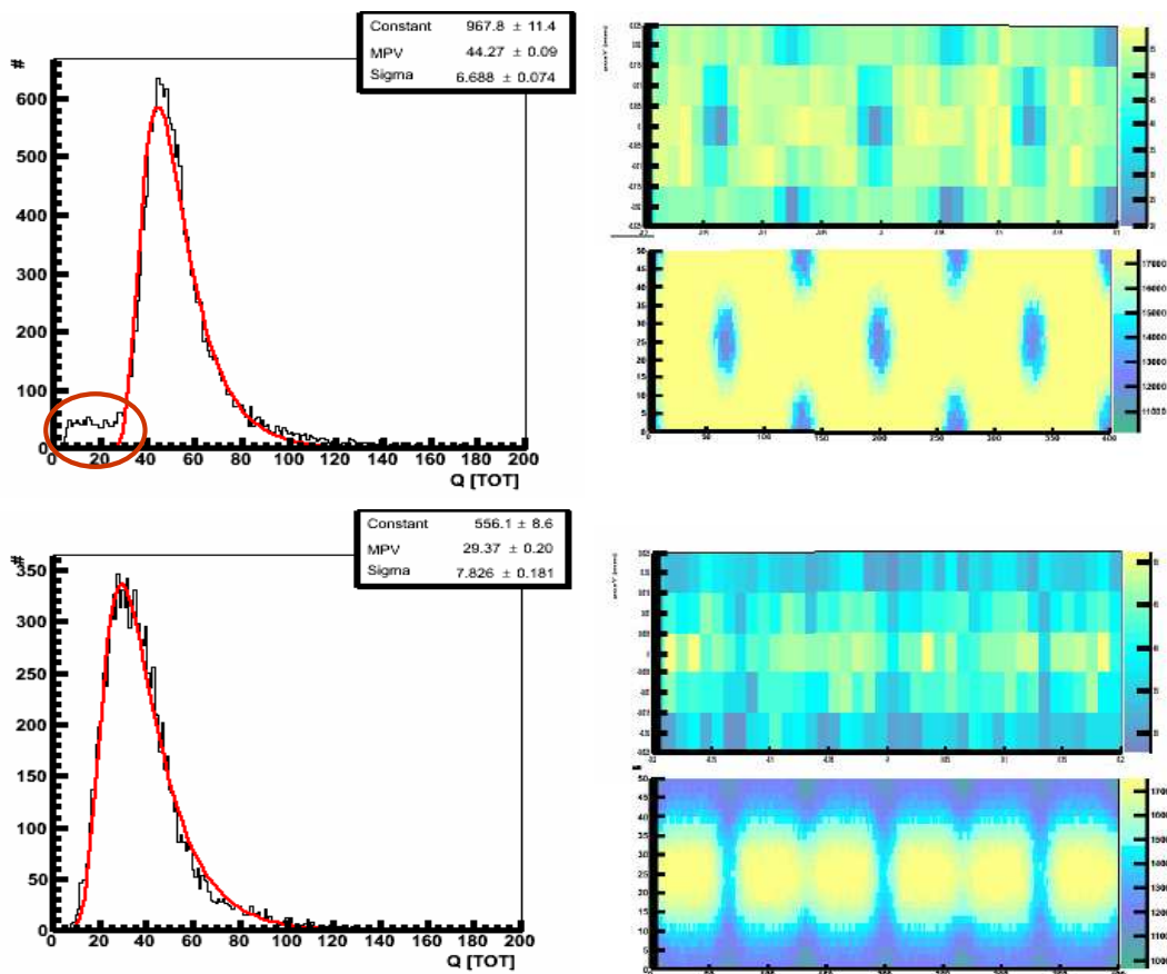
Figure 73. Left: Pulse height spectrum for 100 GeV/c pions incident perpendicularly (top) and at a 15^\circ angle (bottom) on a 3E-3D detector biased at 20 V. One Q[TOT] ADC count is 600 electrons. The threshold was 3200 electrons. The tracking efficiencies are 95.9% and 99.9% respectively. This takes into account the partial response of the central part of the electrodes. Right: Simulations (bottom) are in good agreement with the experimental results (top) [M. Mathes, Bonn].
