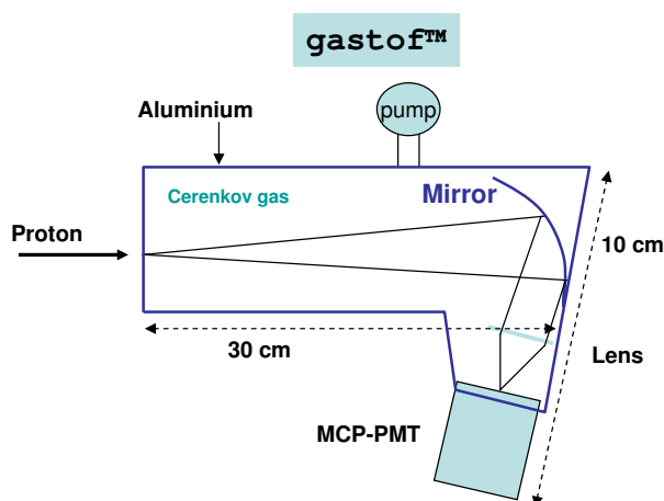
Figure 114. Schematic of GASTOF, a gas-based Čerenkov counter proposed by Louvain-la-Neuve, as described in the text.
