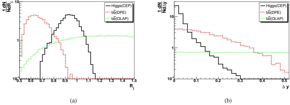
Figure 18. The R_j and \Delta y distributions are shown in (a) and (b) respectively for the signal, [p][b\bar{b}][p] and DPE [p b\bar{b} p] backgrounds. The distributions were reconstructed using a cone radius of 0.7 after smearing the particles with detector resolution.
