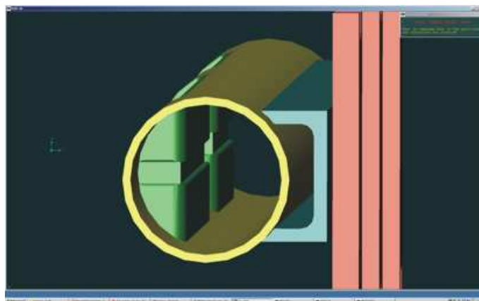
Figure 52. Interior of the moving beam-pipe as seen by the particles.
