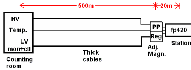
Figure 100. Low- and high-voltage supplies in counting room using 500 m long cables to a patch panel with regulators next to the cryostat. “Station” indicates the FP420 cryostat and “Adj. Magn.” the magnets adjacent to the FP420 cryostat. “PP” is a patch panel. “Reg” indicates linear regulators next to the load.
