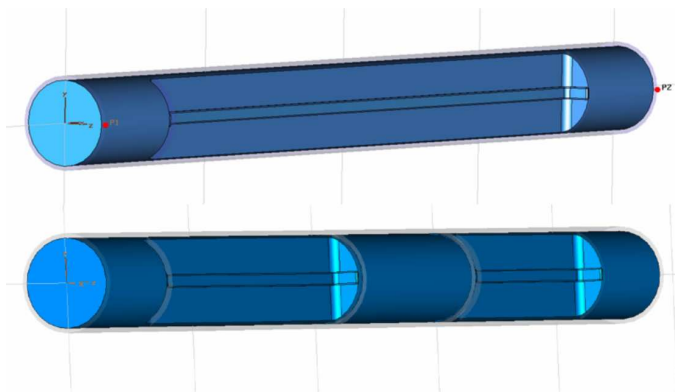
Figure 59. The two benchmark FP420 pocket designs. The upper figure is a single pocket solution. The lower figure is a double pocket design, which will allow separate temperature and vacuum conditions for timing and silicon detectors
