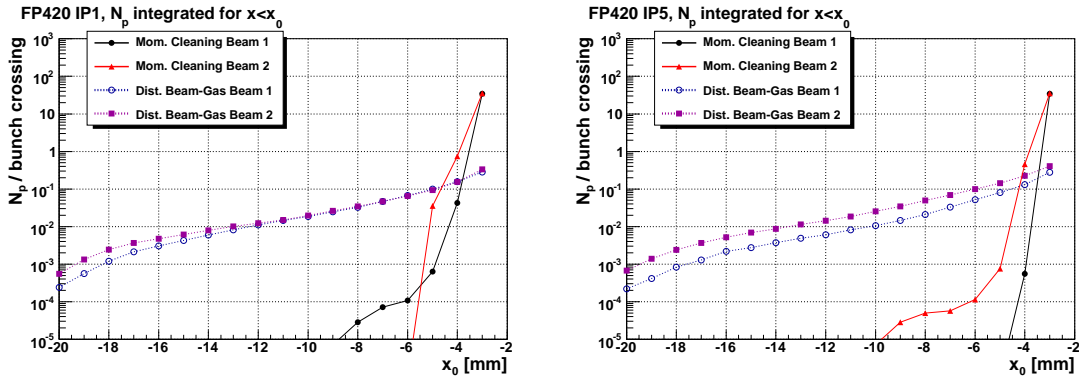
Figure 40. Total amount of beam halo protons predicted at the 420 m regions for different FP420 detector horizontal positions.
