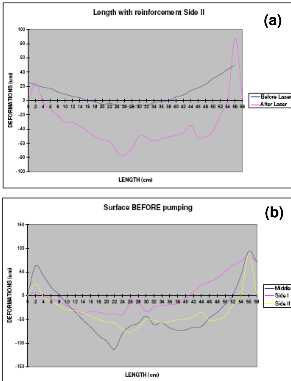
Figure 55. (a) Deformation as a function of length at the “Side 2” location before (blue) and after (pink) laser welding. (b) Deformation after welding but before vacuum pumping for the three locations.
