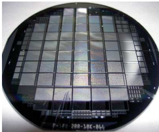
Figure 71. Four-inch wafer processed for the FP420 project. This has 32 3E, 6 4E and 6 2E ATLAS pixel readout compatible devices and several test structures. The 250 micron substrate is 12\ \text{k}\Omega\ \text{cm} p-type.
