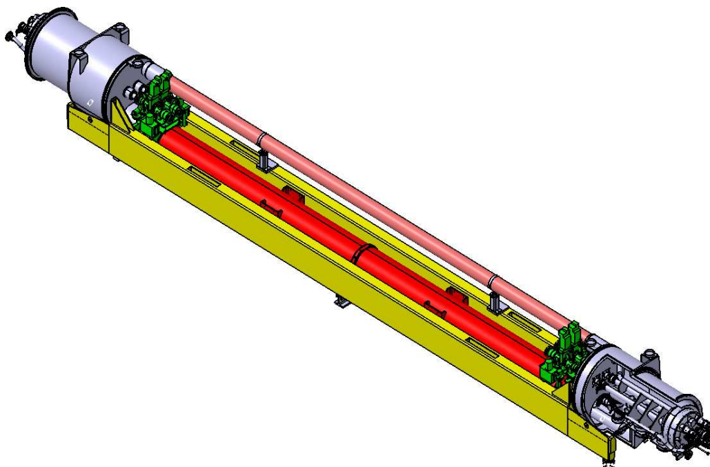
Figure 46. The new connection cryostat for FP420
