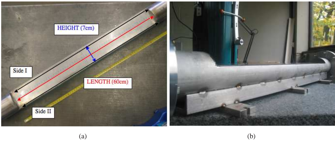
Figure 54. Hamburg pipe prototypes: (left) view of a 600 mm long pocket, laser welded in a tube without reinforcement; (right) picture of a 600 mm long pocket welded by laser in a reinforced tube.
