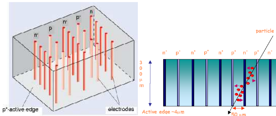
Figure 65. Isometric and lateral view sketches of a 3D detector where the p+ and n+ electrodes are processed inside the silicon bulk. The edges are trench electrodes (active edges) and surround the sides of the 3D device making the active volume sensitive to within a few microns of the physical edge.
