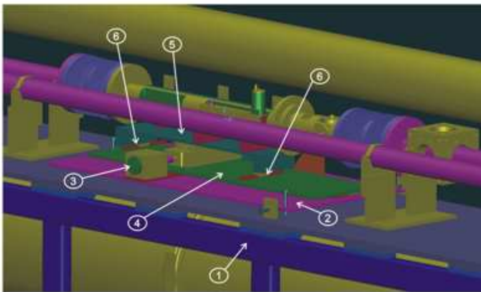
Figure 51. Support table (1), drive support table with alignment system (2), drive motor (3), intermediate table for emergency withdrawal (4), moving support table (5), and linear guides (6).
