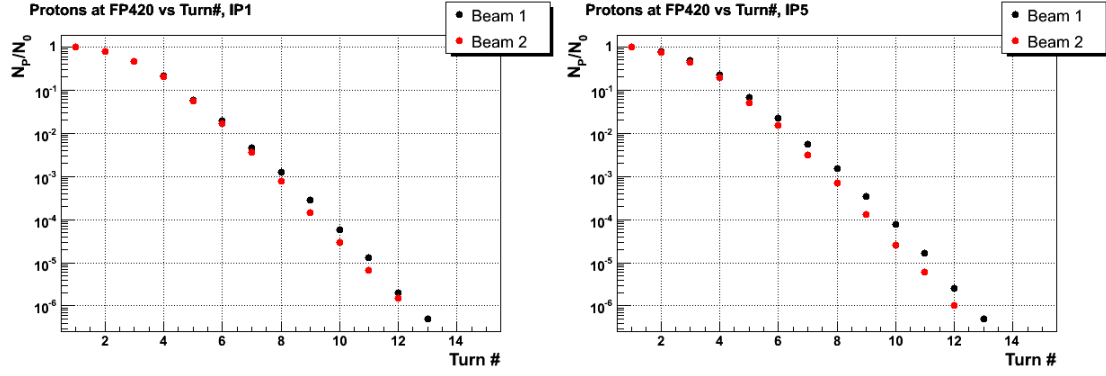
Figure 34. Total number of particles at FP420 as a function of the turn number after scattering on the momentum cleaning collimators.
