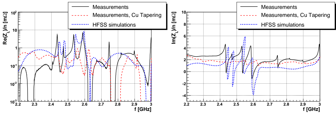
Figure 61. Measurements of real (left) and imaginary part (right) of the longitudinal impedance with the beam 3 mm from the pocket wall for the single pocket prototype; also shown are the HFSS simulations.
