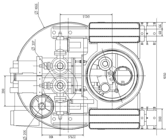
Figure 47. Cross-section view of the new connection cryostat for FP420
