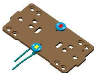
5. Chips 3&4 on second transfer chuck
