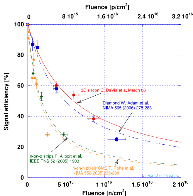
Figure 68. Signal efficiency of 3D detector versus fluence of 1 MeV equivalent neutrons/cm 2 . Data for n on p silicon strips and n-side readout pixel detectors are shown for comparison. Diamond detector results are also shown. Note that diamond gives a factor three less signal for a minimum ionising particle.
