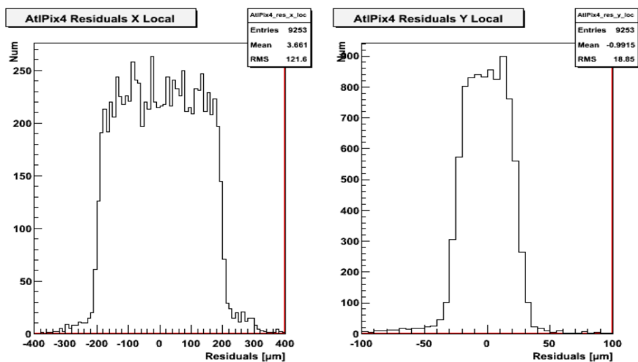
Figure 74. Tracking residuals for 3D pixel detector [M. Mathes, Bonn].
