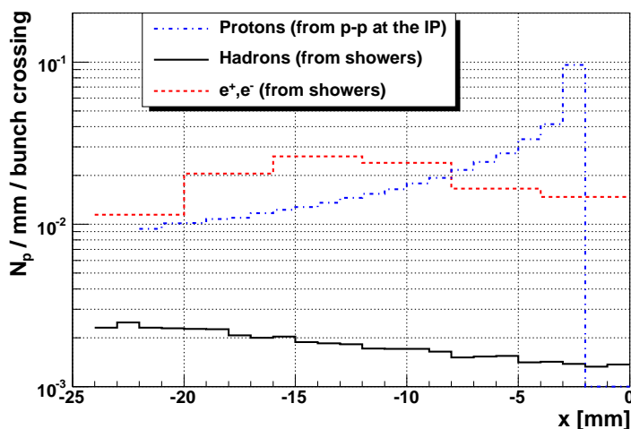
Figure 44. Secondary particles flux at the entrance of the 420 m region downstream of IP5 (preliminary results). The shower source is diffractive protons, generated with DPMJET, lost on the last bending magnet before FP420. The surviving diffractive protons are shown too.
