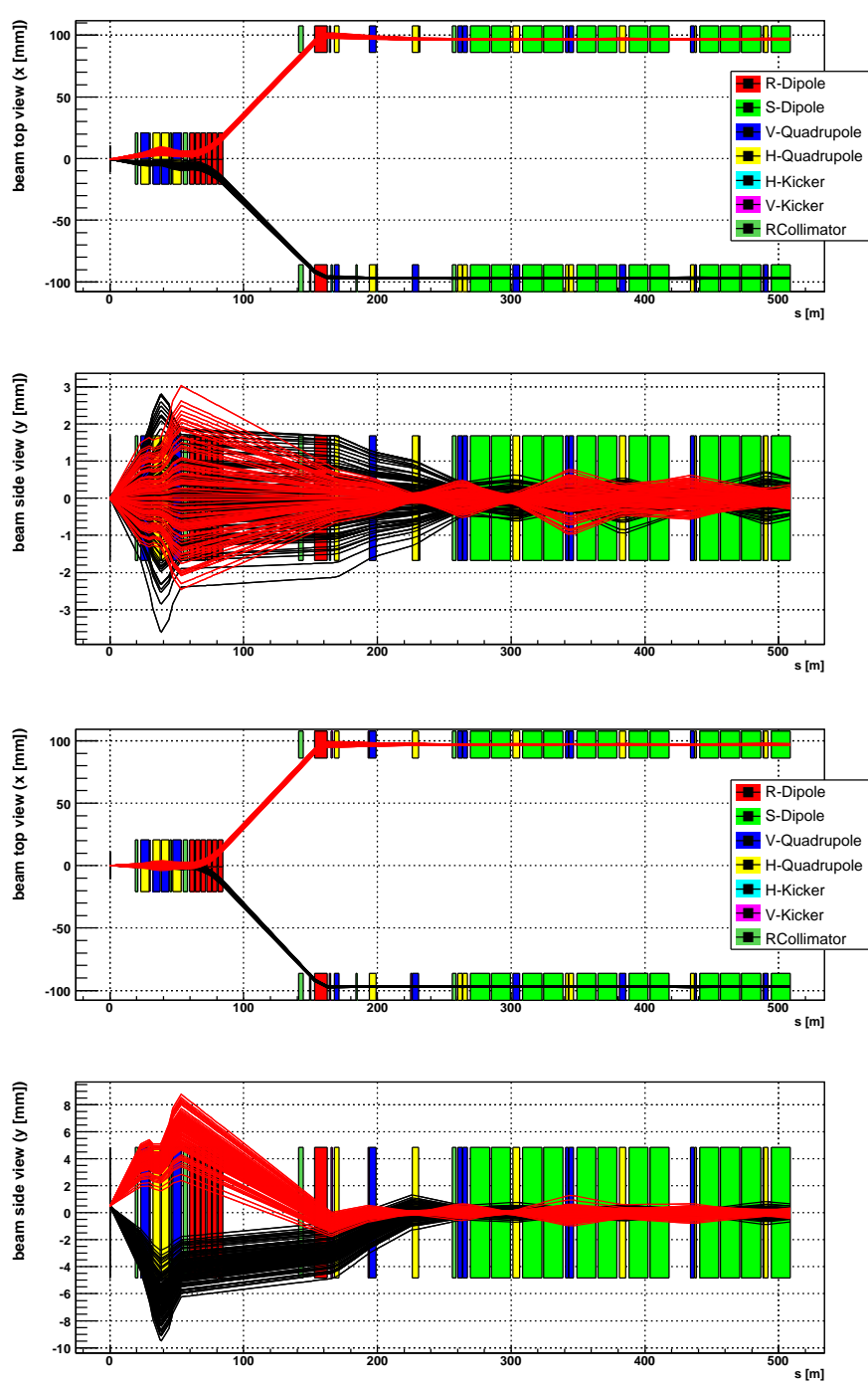
Figure 123. Beam particle paths calculated by HECTOR [61], around CMS (top two figures) and ATLAS (bottom two figures). The beam line has been artificially straightened through the dipole region z > 250 m.
