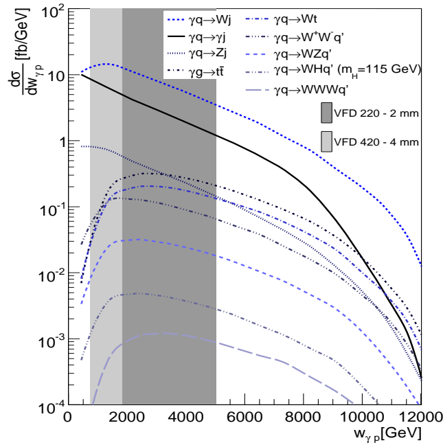
Figure 12. Differential cross-sections for pp(\gamma q/g \rightarrow X)pY processes as a function of the c.m.s. energy in photon-proton collisions, W_{\gamma p} . The acceptance of roman pots (220 m at 2 mm from the beam axis and 420 m at 4 mm from the beam axis) is also sketched [12].
