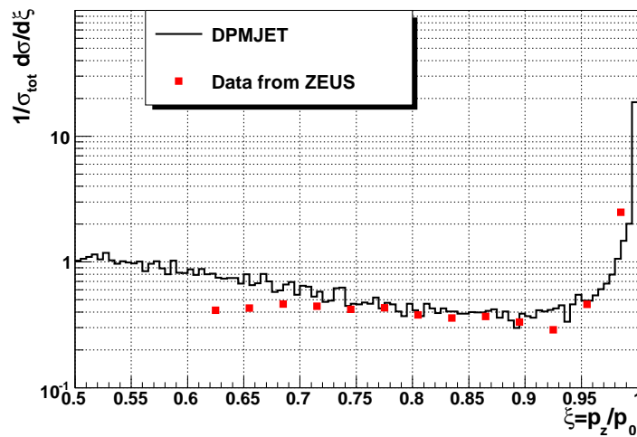
Figure 42. The leading proton spectrum as a function of fractional momentum loss \xi predicted by DPMJET and measured by the ZEUS Collaboration [80].
