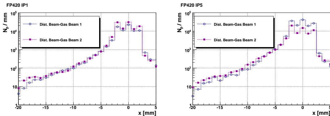
Figure 37. Horizontal distribution of the protons scattered due to beam-gas interaction, as observed at FP420 after the simulation of 1 \cdot 10^7 proton-gas nuclei events per LHC beam.
