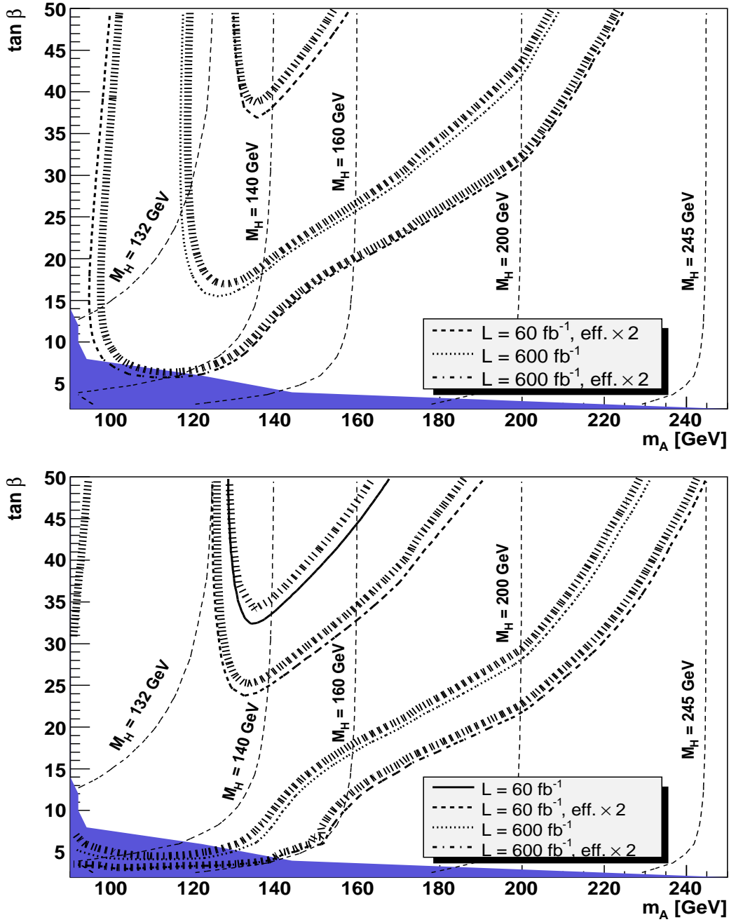
Figure 5. 5\sigma discovery contours (upper plot) and contours of 3\sigma statistical significance (lower plot) for the CEP H \rightarrow b\bar{b} channel in the m_A - \tan\beta plane of the MSSM within the M_h^{\max} benchmark scenario (with \mu = +200\text{GeV} ) for different luminosity scenarios as described in the text [19]. The values of the mass of the heavier CP-even Higgs boson, M_H , are indicated by contour lines. No pile-up background assumed. The dark shaded (blue) region corresponds to the parameter region that is excluded by the LEP Higgs boson searches [42, 43].
