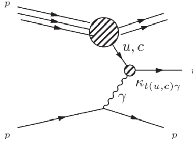
Figure 14. Photo-production of top quarks at LHC through FCNC [12].
