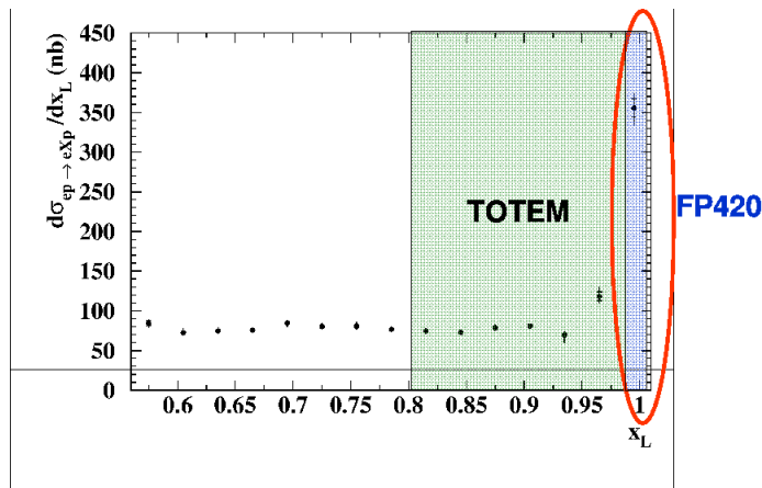
Figure 15. x_L = 1 - \xi coverage of FP420 and TOTEM (or any near-beam detectors at 220 m from the interaction point). The data points are for the reaction ep \rightarrow eXp [80] and are only meant to illustrate the position of the diffractive peak at x_L \approx 1 .
