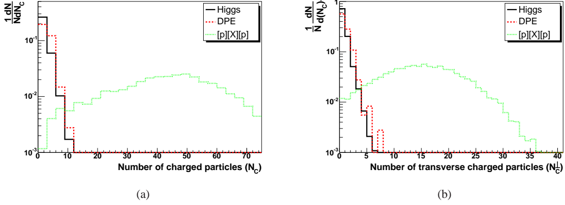
Figure 19. (a) The charged track multiplicity outside of the dijet system, N_C . (b) The number of charged particles that are transverse to the leading jet as defined by equation (3.5). In both cases the particles must satisfy p_T > 0.5 \text{ GeV}/c and |\eta| \leq 1.75 . Only 80% of the particles are used, which replicates ATLAS reconstruction efficiency for low p_T tracks.
