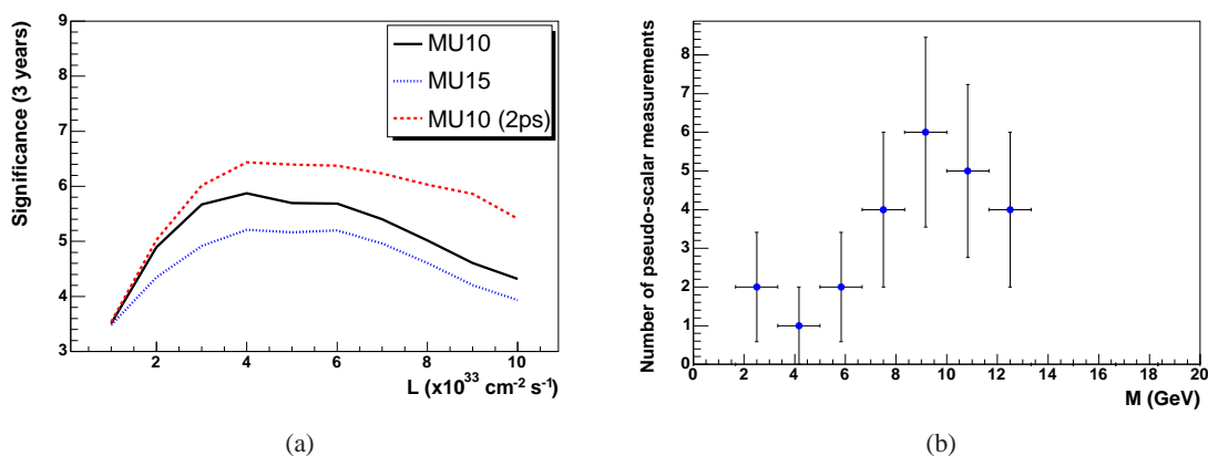
Figure 7. (a) The significance of observation of h \rightarrow aa \rightarrow 4\tau using a muon p_T trigger threshold of 10 GeV/c (or 15 GeV/c) for three years of data taking at ATLAS and CMS. Also shown is the increase in the significance due to a factor of five improvement in background rejection from a 2 ps proton time-of-flight measurement, see sections 3 and 10, or a comparable gain across all of the rejection variables [27]. (b) A typical a mass measurement for 150 \text{ fb}^{-1} of data.
