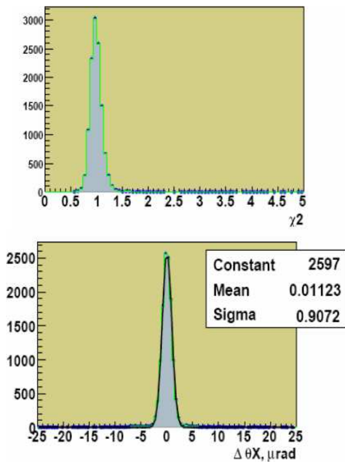
Figure 112. Track \chi^2/\text{NDF} (top) and angular resolution (bottom) for a three-station tracker. The angular resolution is 0.91 \mu\text{rad} if the \chi^2/\text{NDF} is selected to be less than 1.5.
