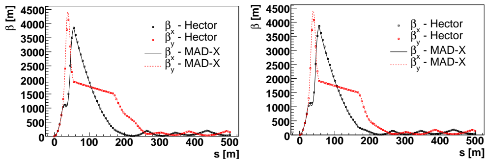
Figure 24. Beta functions \beta_x (horizontal) and \beta_y (vertical) for LHC beam 1 (left) and beam 2 (right) calculated by MAD-X (lines) and HECTOR (squares).
