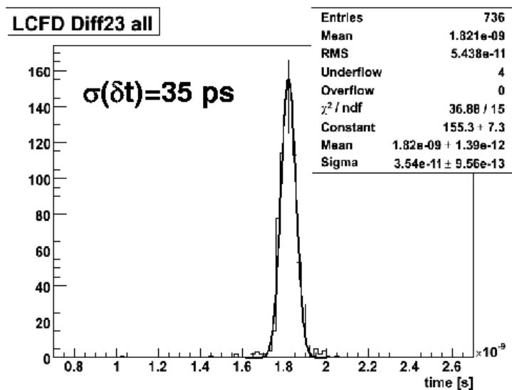
Figure 117. The time difference between the first (G1) and second generation (G2) GASTOF prototype detectors from the March 2007 test beam.
