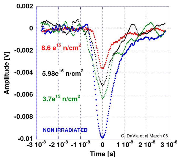
Figure 67. Response of a 3 electrodes/pixel (3E) 3D device to a 1060 nm laser pulse after 3.7 \times 10^{15} , 5.98 \times 10^{15} and 8.6 \times 10^{15} neutrons/cm 2 .
