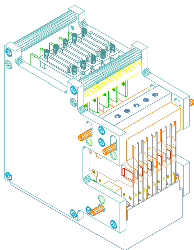
Figure 82. A five superlayer tracking station. The mechanics supports the superlayers and also provides cooling blocks.
