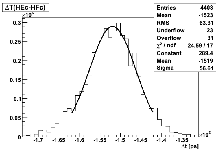
Figure 118. The time difference between two 90 mm long QUARTIC bars as described in text.
