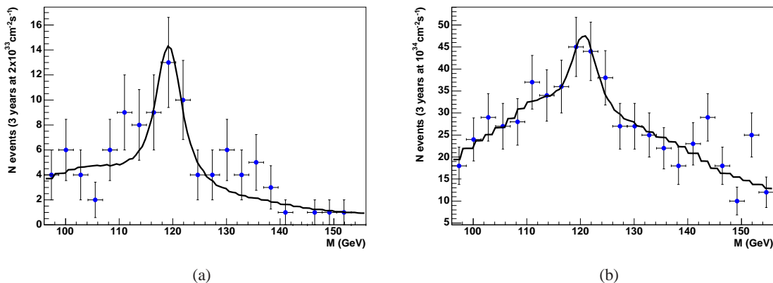
Figure 20. Typical mass fits for the 120 \text{ GeV}/c^2 MSSM h \rightarrow b\bar{b} , with the L1 trigger and analysis cuts discussed in the text, for 3 years of data taking at 2 \times 10^{33} \text{ cm}^{-2} \text{ s}^{-1} ( 60 \text{ fb}^{-1} , 3.5\sigma , left plot) and at 10^{34} \text{ cm}^{-2} \text{ s}^{-1} ( 300 \text{ fb}^{-1} , 3\sigma , right plot).
