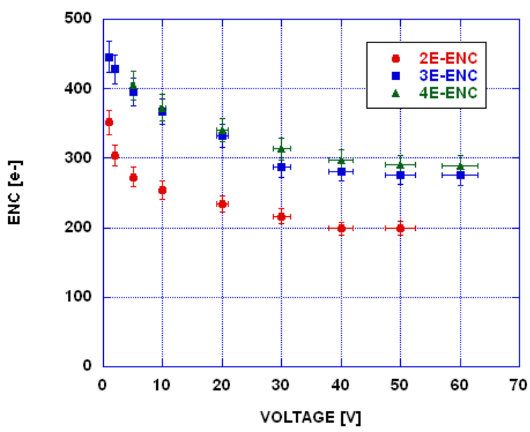
Figure 77. The equivalent noise charge (ENC) of the 2E, 3E and 4E 3D detectors after bump-bonding with the FE-I3 ATLAS pixel readout chip.
