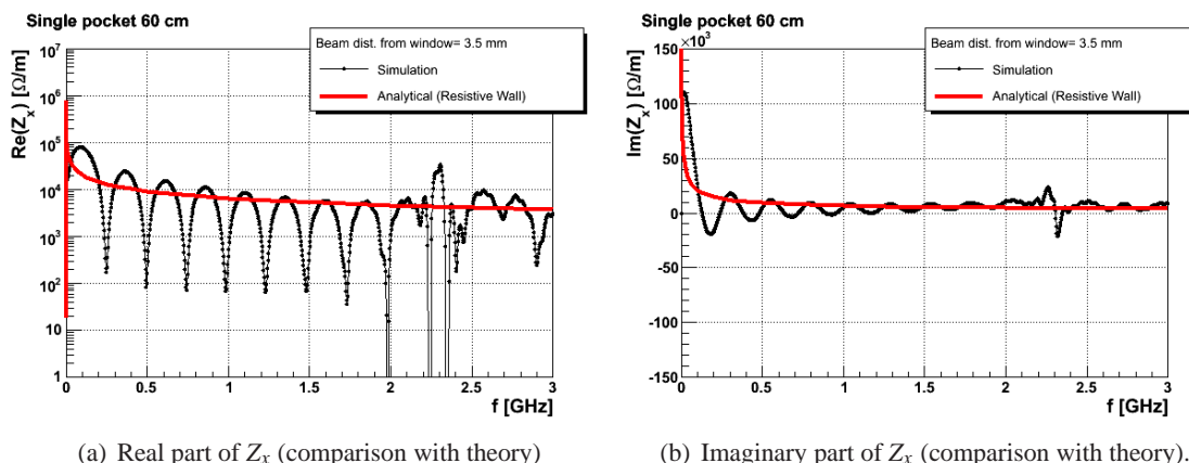
Figure 63. Single pocket transverse impedance vs. resistive wall theory.
