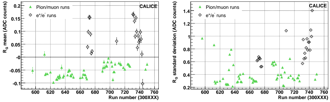
Figure 21. Time dependence of the average over all channels of the residual pedestal R_G : mean value (left) and standard deviation (right) as a function of the run number, for runs taken at CERN in October 2006.
