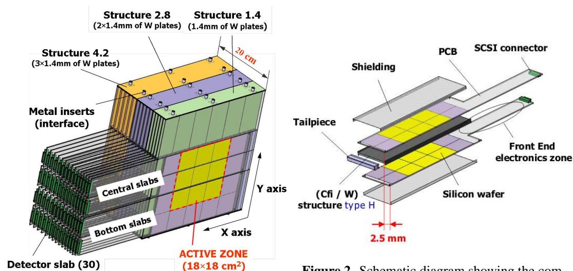
Figure 2. Schematic diagram showing the components of a detector slab.
