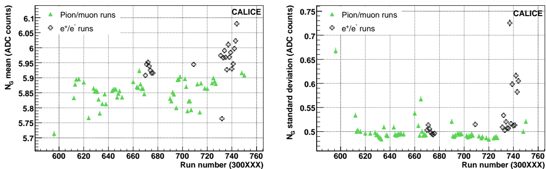
Figure 24. Time dependence of the average over all channels of the noise N_G : mean value (left) and standard deviation (right) as a function of the run number, for runs taken at CERN in October 2006.
