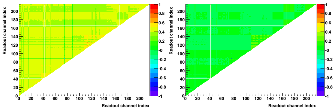
Figure 17. Noise correlation coefficient (colour scale) between all pairs of channels for the VFE PCB situated in the third layer, in a 45 GeV electron run taken at CERN in August 2006, after the simple pedestal subtraction. Left: before correcting the pedestal shifts, the mean correlation is 0.4207 \pm 0.0004 with a standard deviation of 0.0551 \pm 0.0002 . Right: after corrections, the mean correlation is -0.0017 \pm 0.0003 with a standard deviation of 0.0519 \pm 0.0002 .
