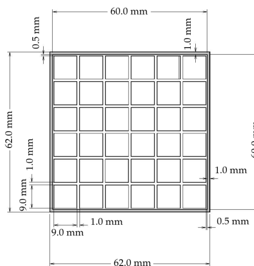
Figure 7. Details of the matrix dimensions in a module (cathode side). The area shaded in grey corresponds to the guard ring.
