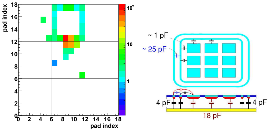
Figure 27. Simple electrical model of capacitive coupling of pads to the guard rings.
