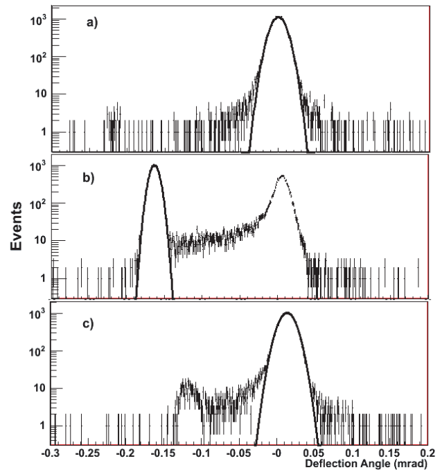
Figure 1: Beam profiles in different crystal positions: a) "amorphous" region, b) "channeling" region, c) volume reflection region.
