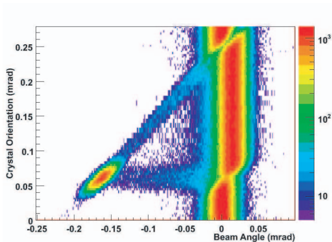
Figure 2: Angular scan of the ST4 crystal selecting only the middle horizontal part of the beam. On the ordinate axis the crystal rotation angle \phi ; on the abscissae axis the particle angle \theta .
