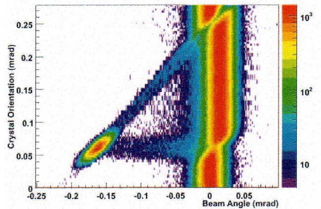
Figure 2: Angular scan of the ST4 crystal selecting only the middle horizontal part of the beam. On the ordinate axis the crystal rotation angle \phi ; on the abscissae axis the particle angle \theta .
