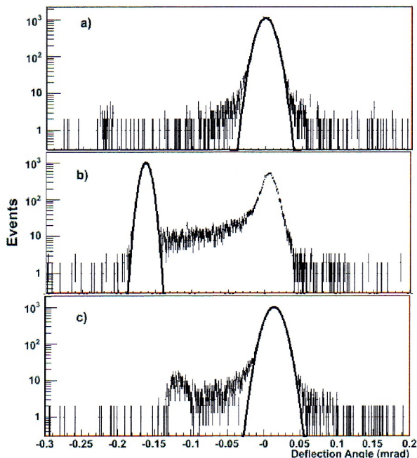
Figure 1: Beam profiles in different crystal positions: a) "amorphous" region, b) "channeling" region, c) volume reflection region.
