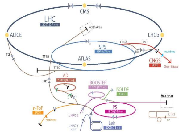
Figure 1: Scheme of the CERN Accelerator Complex
