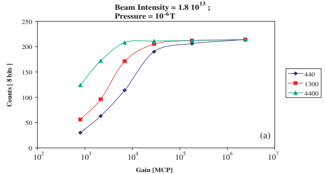
FIG. 10. (Color) CCD counting vs MCP gain for different beam sizes. They decrease as a function of the timing event in the ramp ( T = 440 = larger sizes, T = 4400 = smaller sizes). The figure displays the count variation versus the MCP gain.
