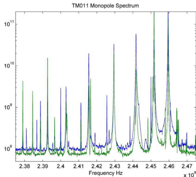
Figure 1. Monopole Spectrum, both couplers
