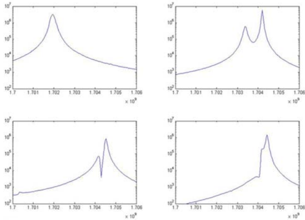
Figure 3 HOM dipole spectra for different cavities showing splitting of polarizations.
