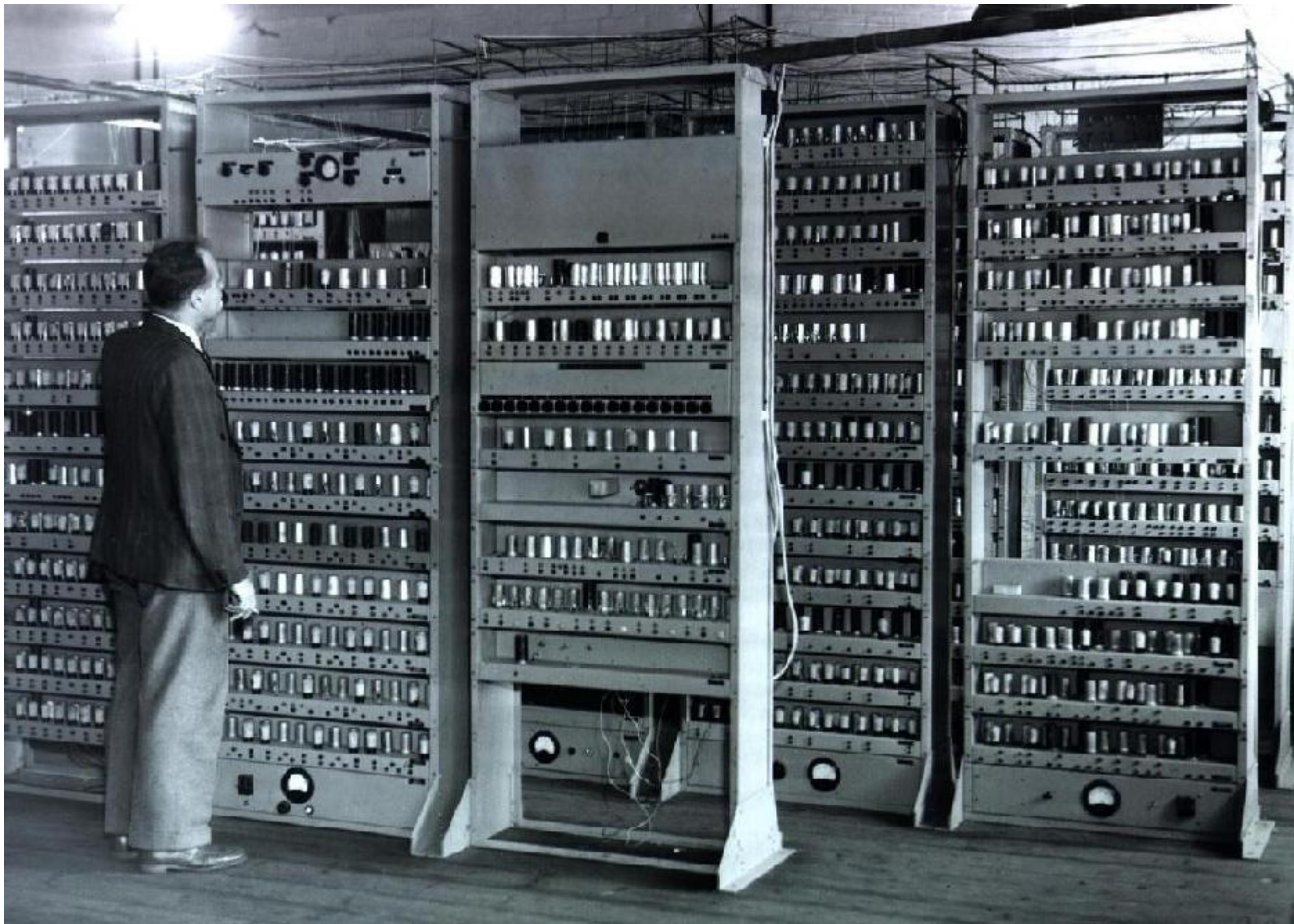
EDSAC 1. Courtesy, Cambridge Computer Laboratory Archive
