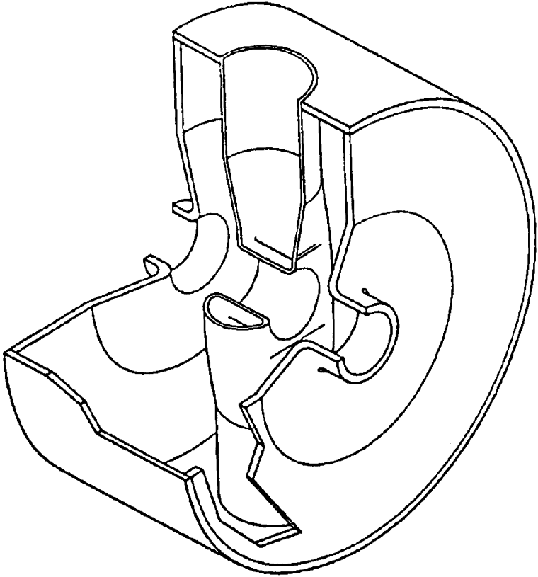
FIGURE 1 A single-cell spoke cavity. The accelerating eigenmode consists of the spoke being excited as a half-wave line.
