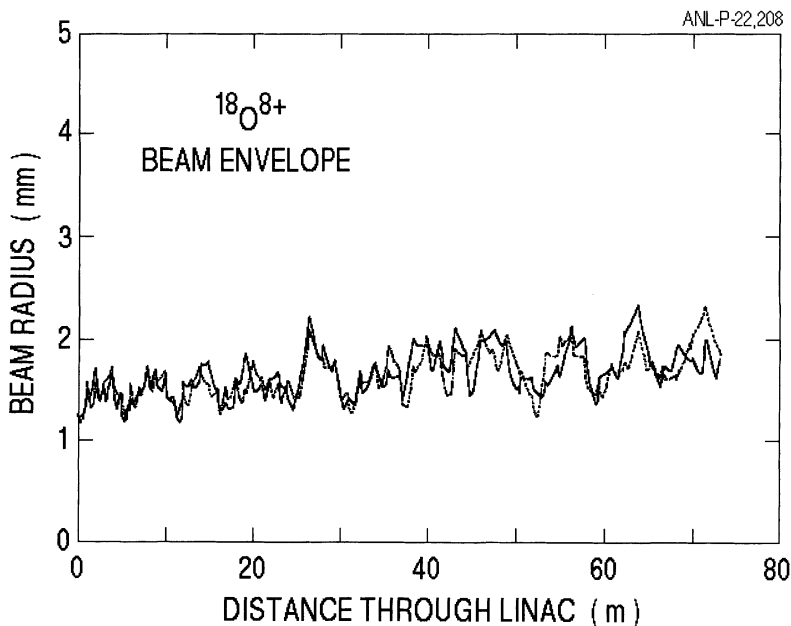
FIGURE 2 Beam envelope for a ^{18}\text{O}^{8+} beam through a 101 cavity array forming a driver linac for a RIB spallation source. For details, see the text.
