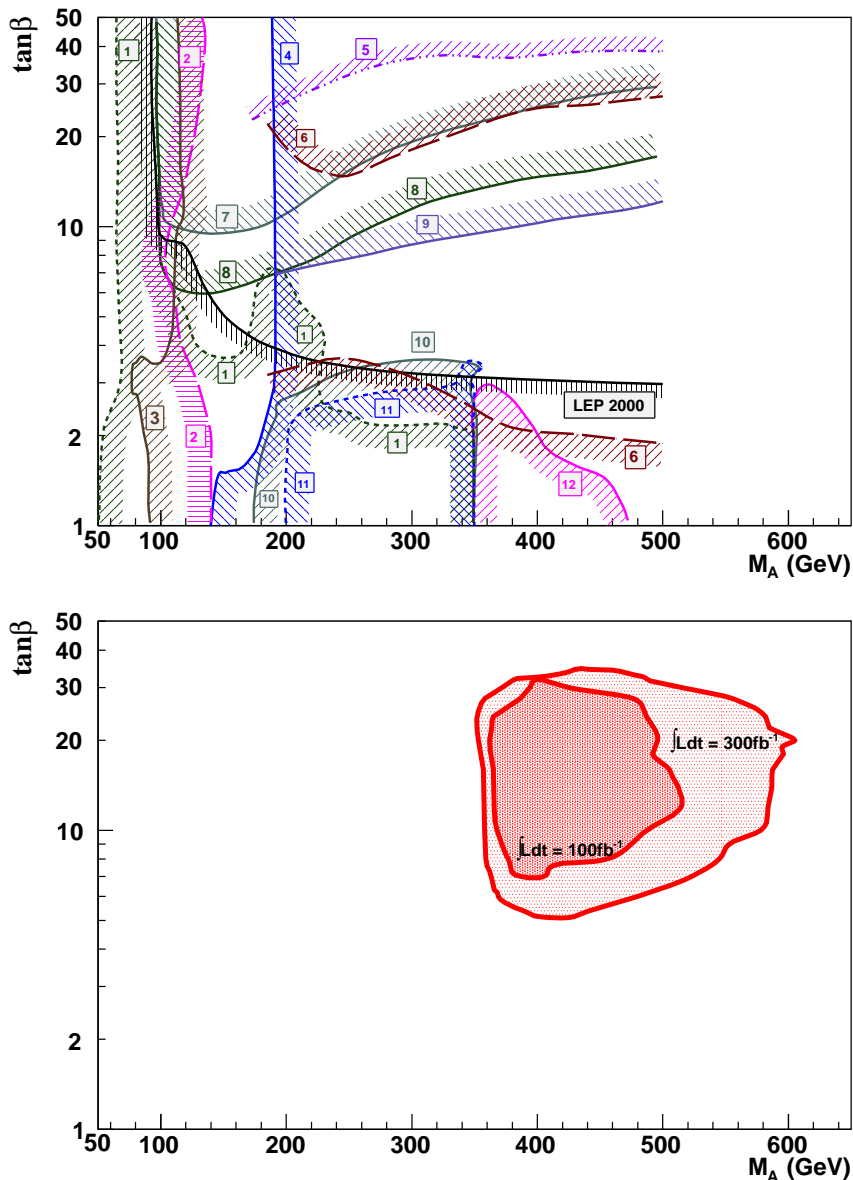
Figure 11. Discovery regions in the (M_A, \tan\beta) plane, here with a logarithmic \tan\beta scale, assuming MSSM Parameter Set 1 –ino inputs and for \mathcal{L}_{\text{int}} = 100\text{fb}^{-1} and 300\text{fb}^{-1} , for the (lower plot) MSSM Higgs bosons’ 4\ell signals from their decays into neutralino or chargino pairs (here H^0, A^0 decays to \tilde{\chi}_2^0\tilde{\chi}_2^0 totally dominate). This is shown juxtaposed (upper plot) with 300\text{fb}^{-1} regions for MSSM Higgs boson signatures from decays to SM particles based upon LEP results and ATLAS simulations [45], where labels represent: 1. H^0 \rightarrow Z^0Z^{0*} \rightarrow 4 leptons; 2. t \rightarrow bH^+, H^+ \rightarrow \tau^+\nu + \text{c.c.} ; 3. t\bar{t}h^0, h^0 \rightarrow b\bar{b} ; 4. h^0 \rightarrow \gamma\gamma and W^\pm h^0/tth^0, h^0 \rightarrow \gamma\gamma ; 5. b\bar{b}H^0, b\bar{b}A^0 with H^0/A^0 \rightarrow b\bar{b} ; 6. H^+ \rightarrow t\bar{b} + \text{c.c.} ; 7. H^0/A^0 \rightarrow \mu^+\mu^- ; 8. H^0/A^0 \rightarrow \tau^+\tau^- ; 9. g\bar{b} \rightarrow \bar{t}H^+, H^+ \rightarrow \tau^+\nu + \text{c.c.} ; 10. H^0 \rightarrow h^0h^0 \rightarrow b\bar{b}\gamma\gamma ; 11. A^0 \rightarrow Z^0h^0 \rightarrow \ell^+\ell^-b\bar{b} ; 12. H^0/A^0 \rightarrow t\bar{t} . Note that SM discovery regions are not for the same input parameters: they presume a very heavy sparticle spectrum; identical MSSM inputs to those used for the lower plot may well yield smaller SM discovery regions in a revised upper plot. For the 4\ell signals from \tilde{\chi}_i^0\tilde{\chi}_j^0, \tilde{\chi}_m^+\tilde{\chi}_n^- decays, the MSSM Parameter Set 1 –ino/slepton parameters are \mu = -500\text{ GeV}, M_2 = 180\text{ GeV}, M_1 = 90\text{ GeV} and m_{\tilde{\ell}_{\text{soft}}} = m_{\tilde{\tau}_{\text{soft}}} = 250\text{ GeV} .
