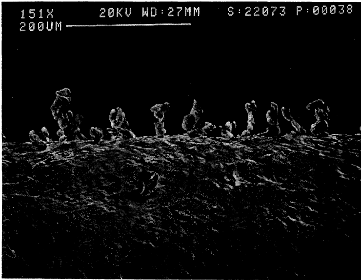
FIGURE 13: Fe particles found vertically aligned on Thomson cavity finger after RF test.
