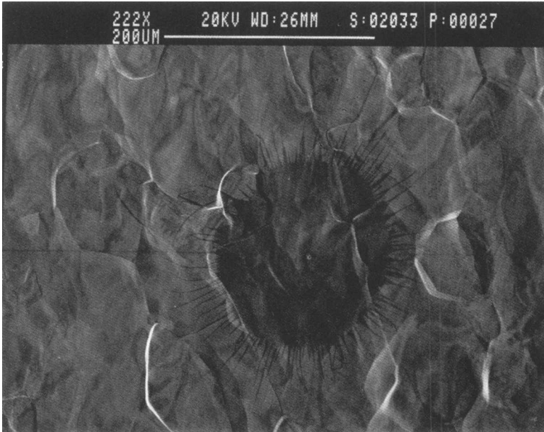
FIGURE 5: Typical starburst, found on mushroom cavity endplate.
