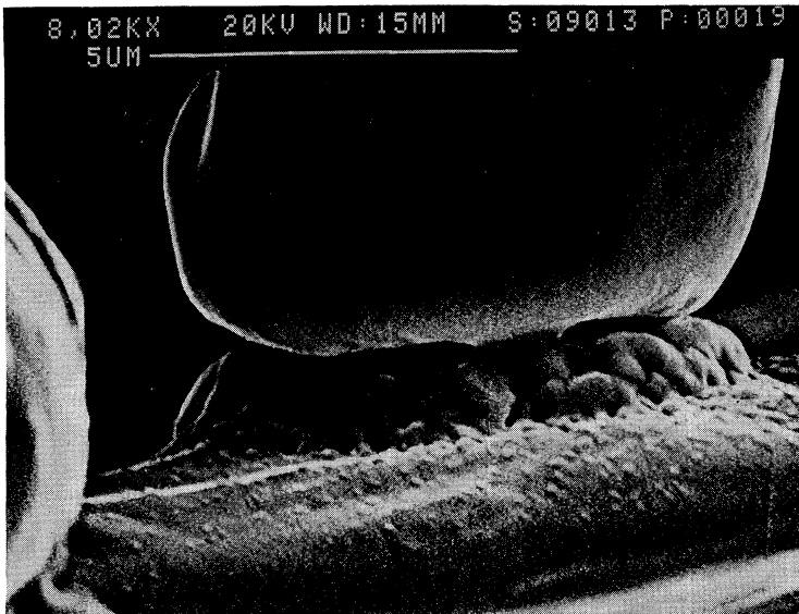
FIGURE 14: Base of Fe particle found welded to Thomson finger surface after RF test.
