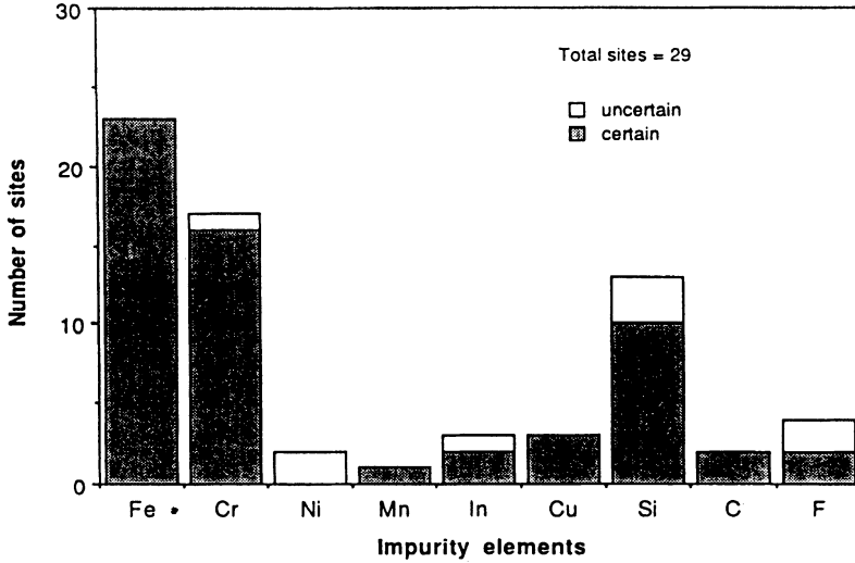
FIGURE 12: Relative frequency of foreign elements found in mushroom cavity craters.
