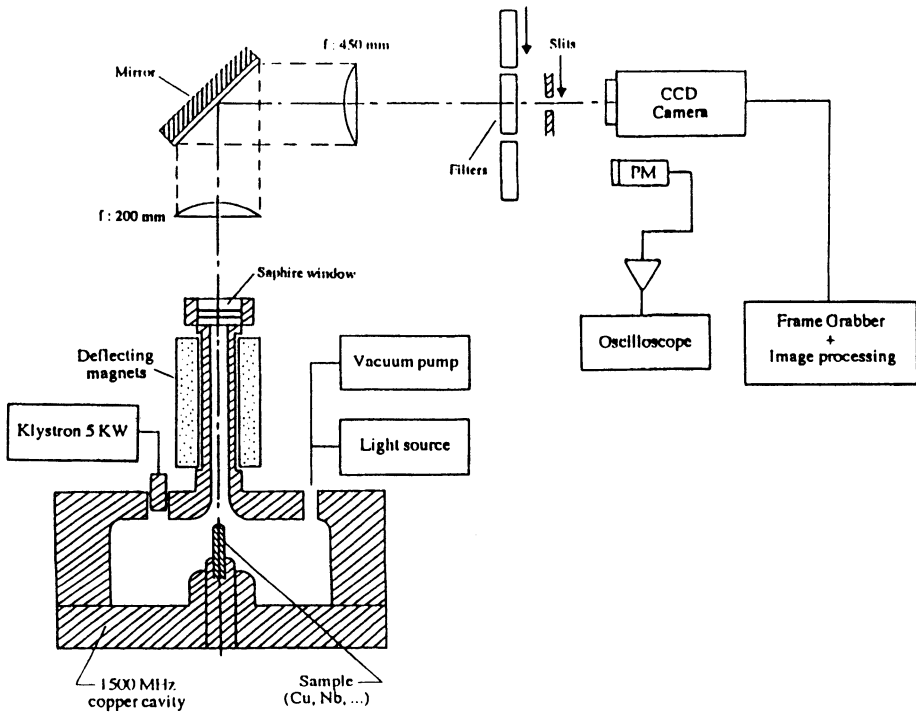
FIGURE 3: Thomson cavity modified for optical measurements.
