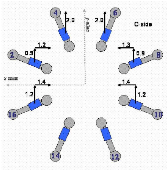
Fig. 17.8: Displacement of the various coils while 21 kA were put in the toroid
