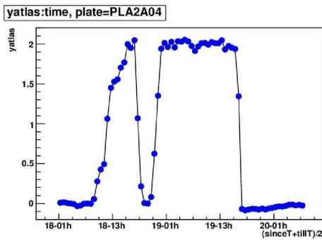
Fig. 17.10: Displacement in mm of the upper coil versus time on November 18th and 19th 2006. Two peaks can be seen, corresponding to two different ramp-ups. The end of the second peak corresponds to a fast quench of the toroid system.
