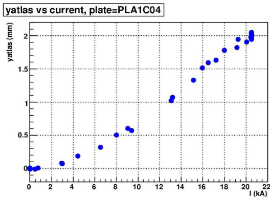
Fig. 17.9: Displacement of the upper coil versus the current in the toroid
