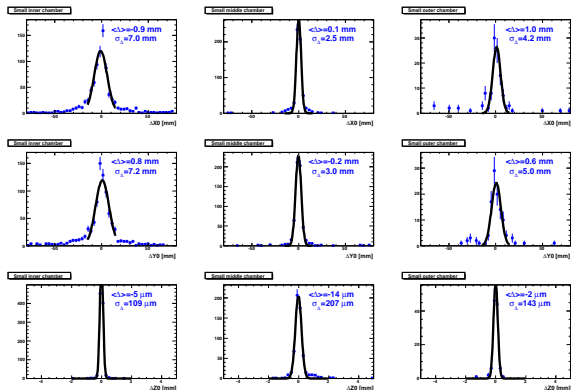
Fig. 17.5: The accuracy of the pseudo-track-sensors
