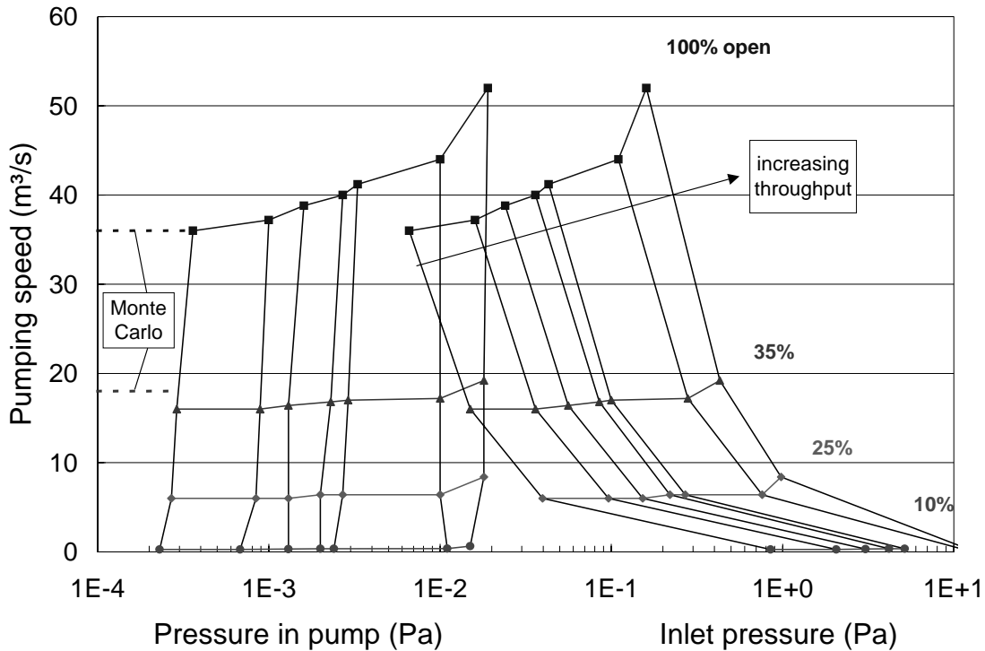
Fig. 20: Pumping characteristics of the model pump. Results for a typical fusion exhaust model gas, consisting of 87% D 2 , 10% He, and 3% impurities (CO, CH 4 , CO 2 , O 2 ). The throughput was varied [between 6 \times 10^{-6} \text{ Pa} \cdot \text{m}^3/(\text{s} \cdot \text{cm}^2) and 4 \times 10^{-4} \text{ Pa} \cdot \text{m}^3/(\text{s} \cdot \text{cm}^2) ] at constant valve position (100%, 35%, 25% and 10% open).
