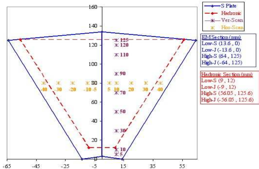
Figure 5: Projection of the EM (blue) and HAD (red) sections onto a 45^\circ plane. The numbers indicate the x - y coordinates of the beam impact points (indicated by the 'x' symbol) used in the horizontal and vertical scans.
