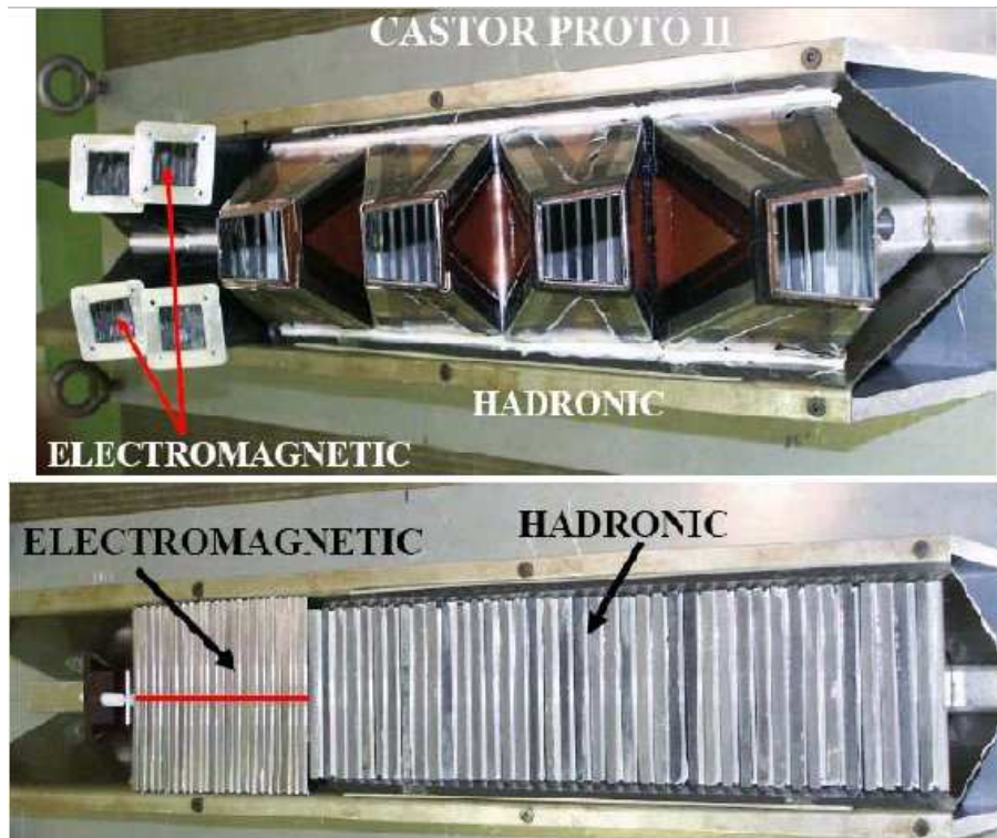
Figure 2: Photographs of the W/Q-plates of the EM and HAD sections (lower picture) and of the light guides (upper picture) in the semi-octant (octant) geometry of the EM (HAD) sections respectively of the CASTOR prototype-II.
