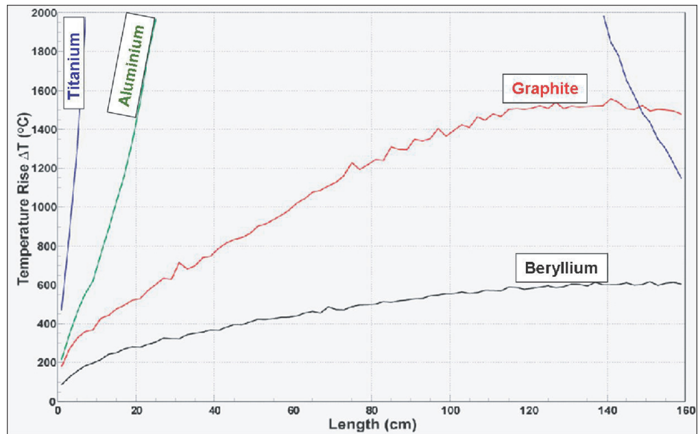
Figure 16. Temperature increase after about 20 bunches at 7 TeV hit the collimators versus length of the jaw (courtesy P Sievers et al 2003 LHC Performance Workshop, Chamonix XII and [6]).
