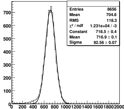
Fig. 2. The sum of the gain corrected signals in the central tower irradiated by 50 GeV/c positrons and the two neighbouring towers.
