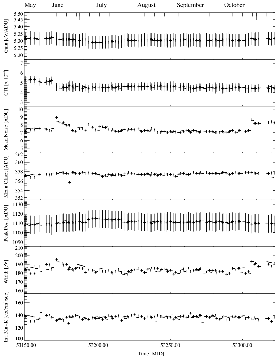
Figure 10. Performance of the pn-CCD of the CAST telescope during the data taking period of 2004. The results are from daily calibration measurements using an ^{55}\text{Fe} source. From top to bottom are shown: The gain of the detector (i.e., ADU to eV conversion), the charge transfer inefficiency (CTI), the mean noise and offset averaged over all 12800 pixels, the peak position, the width (FWHM), and the intensity of the Mn – K \alpha line. The time is given in UT as “Modified Julian Day” (MJD), i.e. \text{MJD} = \text{JD} - 2400000.5 where JD is the Julian Day.
