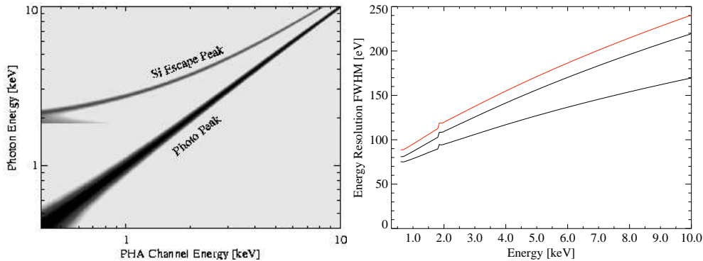
Figure 6. Left: Detector response matrix of the pn-CCD detector. Apparent are the contributions of the photo peak and the Si – K\alpha escape photons. The width of the distribution corresponds to the finite energy resolution of the detector. The color scale is logarithmic. Right: Energy resolution of the CAST pn-CCD and the EPIC-pn detector of XMM-Newton depending on the incident photon energy and different pattern types. From top to bottom: The combined energy resolution of the CAST pn-CCD for single and double event patterns (see text for a more detailed explanation), the energy resolution of the EPIC pn-CCD for double events, and for single events only. The XMM-Newton EPIC pn-CCD data is taken from (Popp et al. 2000) and (Haberl et al. 2002).
