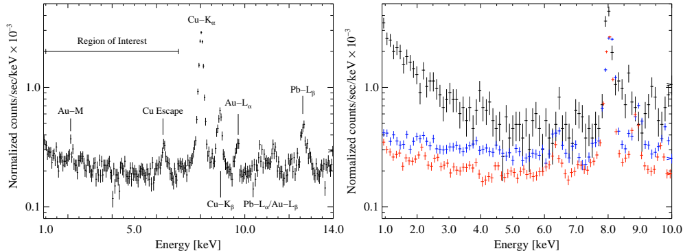
Figure 11. Left: Background spectrum observed during non-tracking times, i.e., while the CAST magnet was not pointing to the sun but under the same operating conditions as during observations of the sun (see Andriamonje et al. 2007). The fluorescent emission lines apparent in the spectrum are labeled. The energy range which is sensitive for axion detection is marked as Region of Interest . Right: Background spectra observed with the pn-CCD under different shielding conditions. From top to bottom: Background observed with the internal copper shield (black), internal copper shield and internal lead shield (blue), and the final shield configuration being installed (red).
