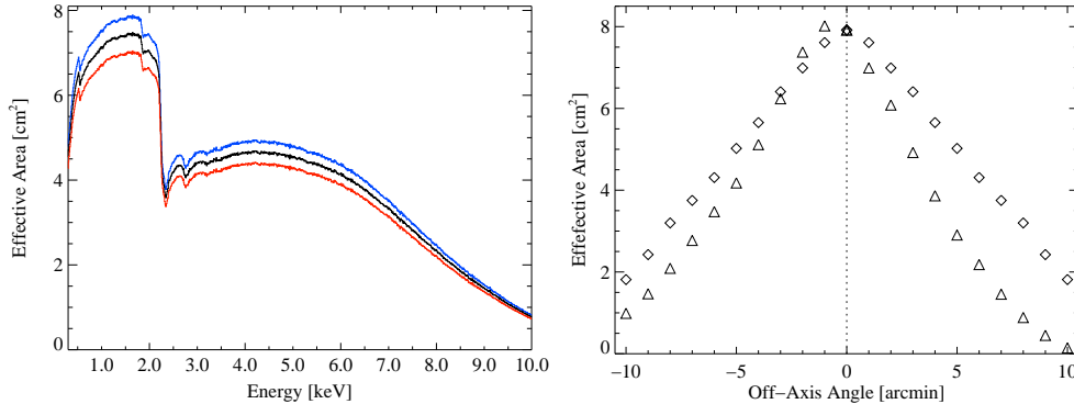
Figure 3. Left: On-axis effective area of the X-ray telescope for a magnet bore aperture with a diameter of d = 43 mm, given by the mirror reflectivity and the quantum efficiency of the pn-CCD. Three different cases are shown: the effective area of the mirror system for a point source for the data taking period of 2003 (blue line), the effective area for a point source located at an infinite distance for the data taking period of 2004 (black line), and for a source of the angular size of the axion emission region on the sun for the data taking period of 2004 (red line). Right: Off-axis behavior of the effective area of the mirror system only, for the data taking period of 2003 is shown for two cases: for radial off-axis angles (triangles) and tangential off axis angles (diamonds). For a more detailed explanation see text.
