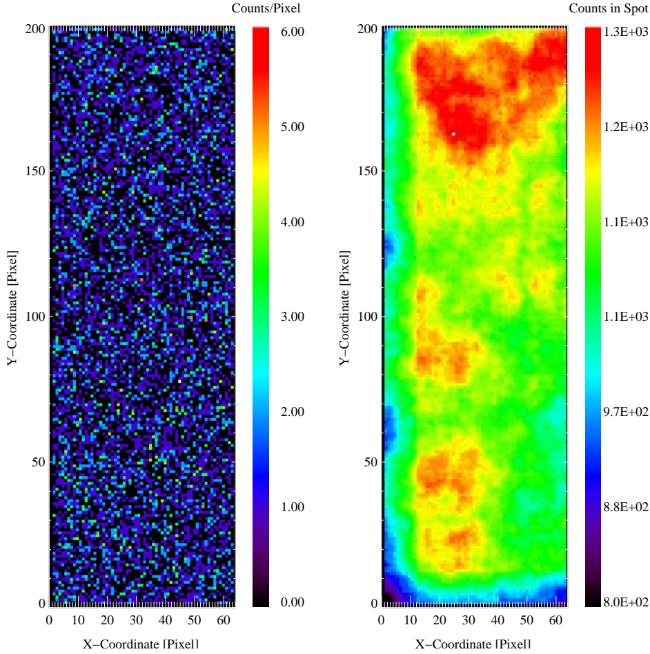
Figure 12. Left: Background spatial distribution as observed by the CAST X-ray telescope during the 2004 data taking period. The intensity is given in counts per pixel and integrated over the full observation period of t_{\text{obs}} = 6805 ksec. Right: The same data smoothed with a circular spot of the size of the expected axion image of the sun.
