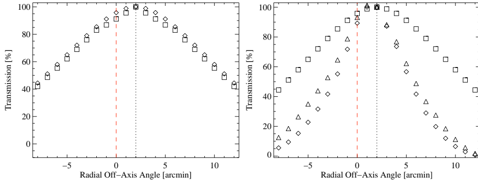
Figure 4. Left: Vignetting losses due to the magnet bore geometry are shown for two cases: a point like source (diamonds) and an extended source of the angular size of the axion emission region on the sun (rectangles). Right: The transmission of the individual components (magnet bore, mirror system) depending on the off-axis angle. This includes the vignetting losses due to the magnet bore (rectangles), the radial off-axis transmission of the mirror module (triangles), and the total transmission of the whole system including both components (diamonds, a more detailed explanation is given in the text).
