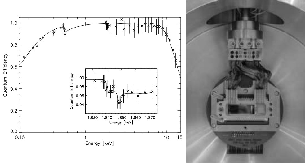
Figure 5. Left: Quantum efficiency (QE) of the fully depleted pn-CCD as measured for the EPIC pn-camera of XMM-Newton (Strüder et al. 2001). The drop of the QE at 0.53 keV is due to absorption losses in the SiO 2 passivation layer at the detector surface. The inset shows the absorption fine structure close to the Si-K edge at 1.84 keV. The solid line represents a detector model fit to the measurements. Right: The focal plane pn-CCD detector inside the CAST telescope. The gold plated cooling mask surrounding the rectangular pn-CCD chip (black part in the center) is connected to a cold finger of a Stirling cooler on the top of the detector chamber via flexible copper leads. Electrical connections to the printed circuit board behind the CCD chip are provided via the flex-lead leaving the chamber on the bottom. The internal Cu/Pb shield is removed in this picture.
