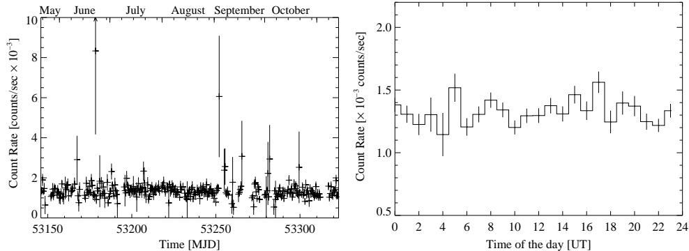
Figure 13. Left: Time dependence of the background in the CAST axion sensitive energy range from 1 to 7 keV observed during the data taking period of 2004. The time is given as MJD (UT). Right: Temporal behavior of the background during the course of one day in the energy range from 1 to 7 keV
