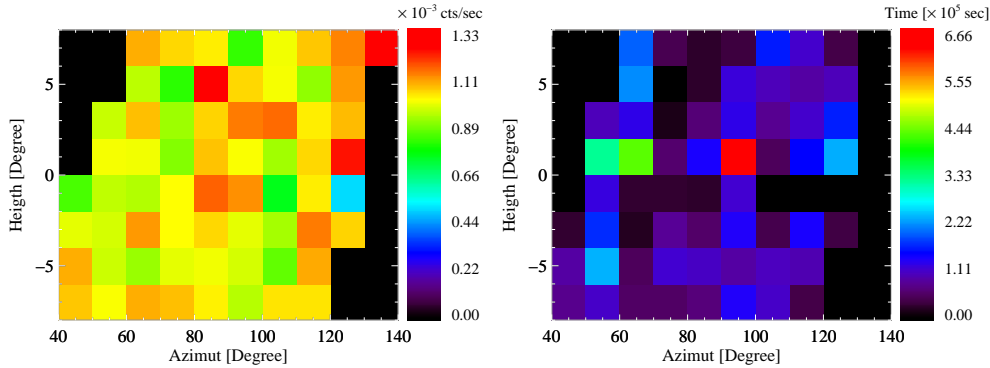
Figure 14. Left: Count rate observed with the X-ray telescope depending on the pointing direction of the magnet. Each cell has a dimension of 10^\circ \times 2^\circ . Right: Integration time for each cell.
