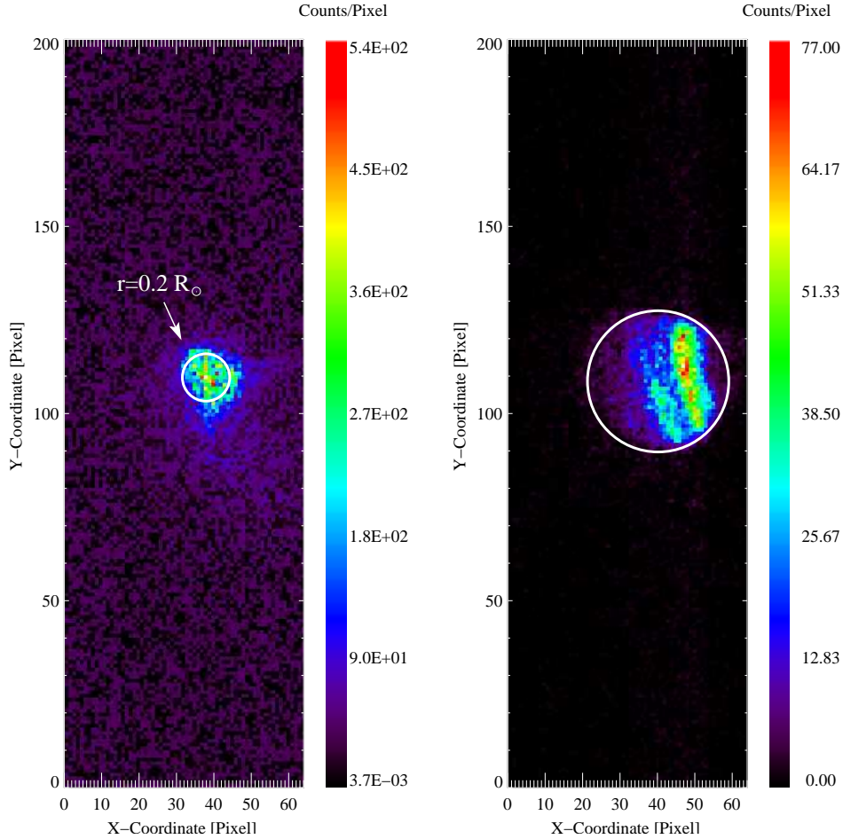
Figure 8. Left: The focal plane intensity distribution of the parallel laser beam, defining the location where an axion signal would be expected. For comparison the size of the axion image of the sun is indicated by a circle with a radius of \approx 0.2R_{\odot} . Right: The focal plane intensity distribution of the 8 keV X-ray photons emitted by the pyroelectric X-ray source. The circle marks the size of the magnet bore projected to the focal plane of the mirror system. The position of the laser spot (center of the circle in the image on the left side) has to coincide with the center of this circle.
