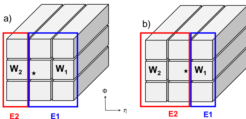
Figure 8. Definition of E1 and E2 when a) W_1 < W_2 and b) W_1 > W_2 (see text). The star represents the electron's incident position.
