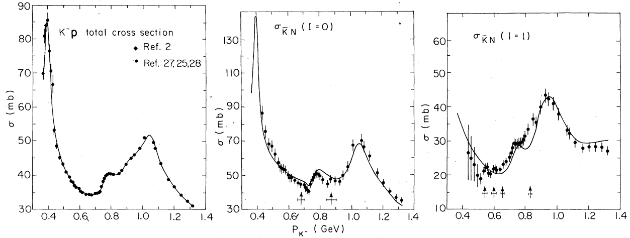
FIG. 7. The total K^-p cross sections and the I=0 and I=1 cross sections used in this analysis compared with our fit. The arrows indicate the locations and widths of six new resonances claimed by Carroll et al. (Ref. 27).
