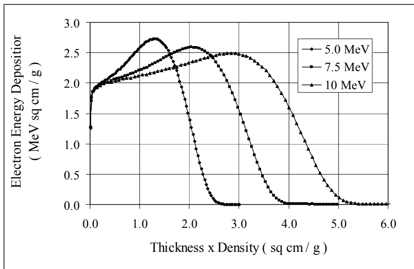
Fig. 4: Electron energy deposition vs thickness x density in polyethylene at 5.0, 7.5 and 10 MeV incident electron energy. The beam window thickness is 40 um of titanium. The air thickness between the window and the treated material is 15 cm at 0.0012 g/cu cm. From Refs. [74, 75].
