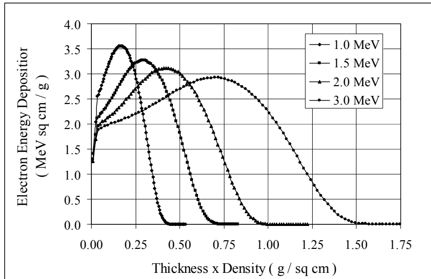
Fig. 3: Electron energy deposition vs thickness x density in polyethylene at 1.0, 1.5, 2.0 and 3.0 MeV incident electron energy. The beam window thickness is 40 um of titanium. The air thickness between the window and the treated material is 15 cm at 0.0012 g/cu cm. From Refs. [74, 75].
