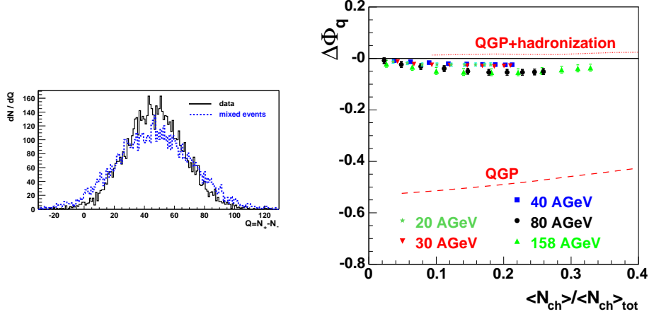
Fig. 15. Left: Distributions of net charge Q = N^+ - N^- for the rapidity range -1.4 < y < 2.4 in central Pb+Pb collisions at 158A GeV for data (full histogram) and mixed events (dotted histogram). Right: Measure \Delta\Phi_q of electric charge fluctuations corrected for charge conservation versus rapidity acceptance.
