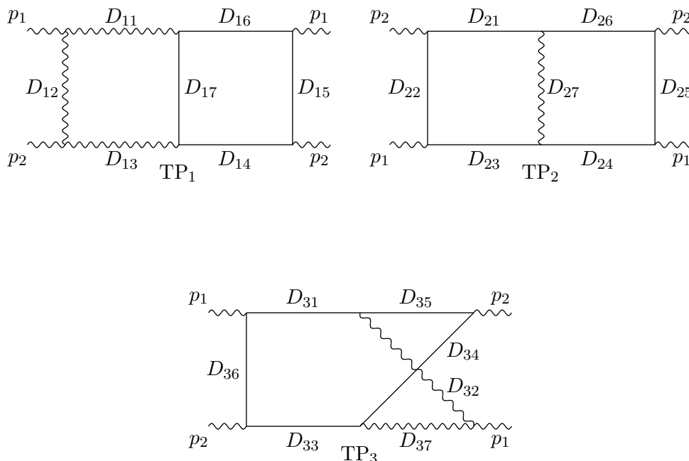
Figure 2: Master topologies. Wavy lines denote massless particles both external and internal. Internal massive lines are denoted by single straight lines whereas the double line denotes a massive external particle.
