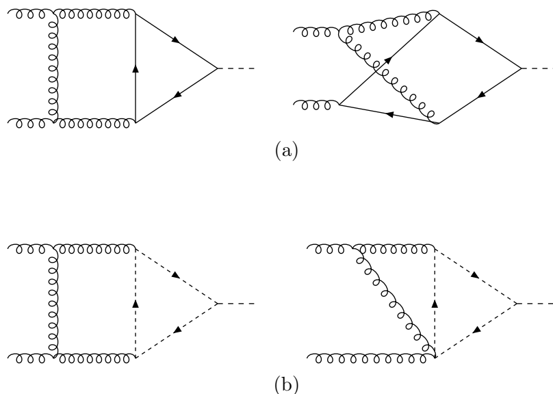
Figure 1: Typical Feynman diagrams in the two loop contributions to gg \rightarrow H with (a) a heavy fermion in the loop, (b) a heavy scalar in the loop .
