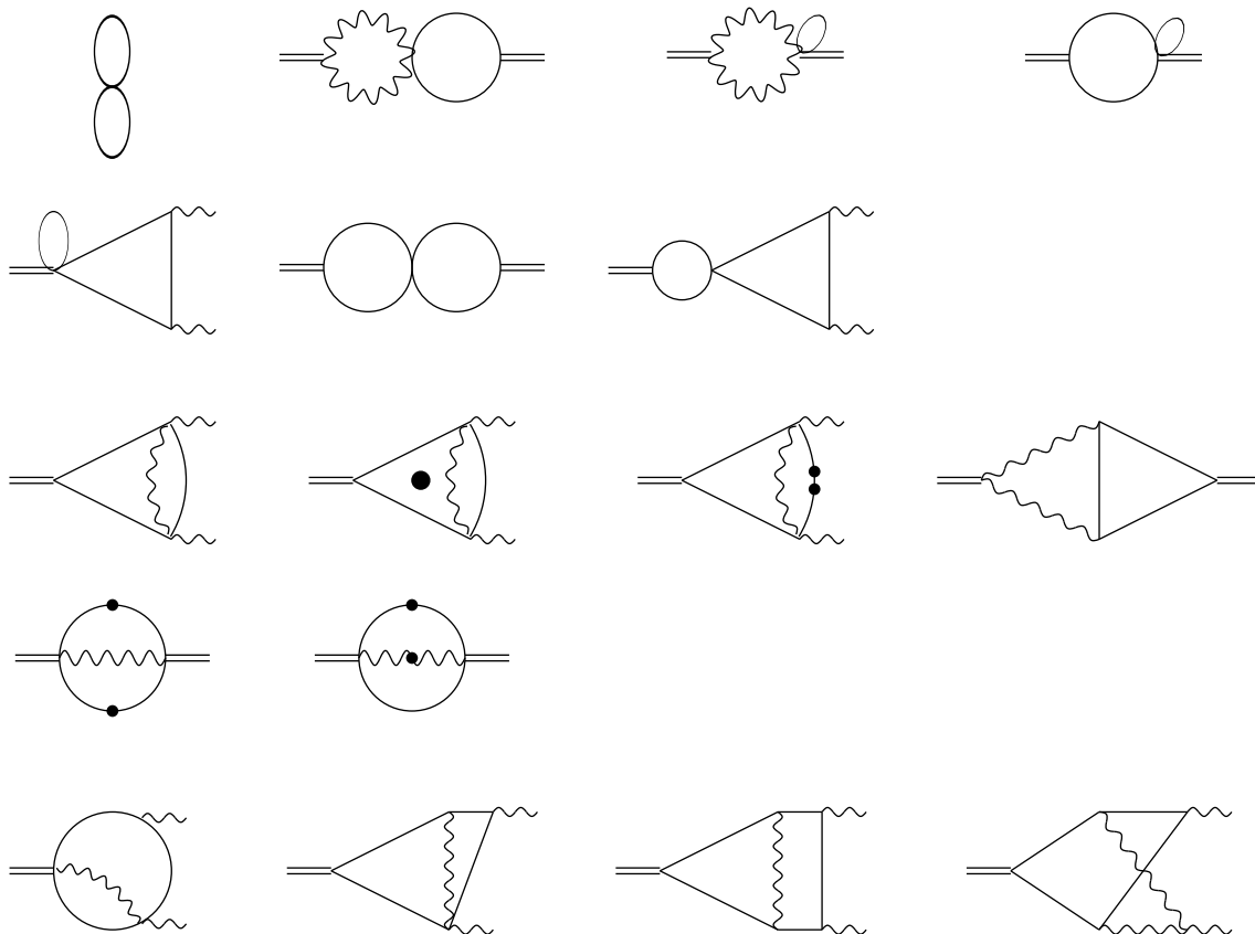
Figure 3: Set of master integrals. The conventions for the lines are as in figure 2. Each dot on a propagator line denotes an additional power of the propagator in the denominator. The diagram with a big dot contains a numerator, it is defined in the following section.
